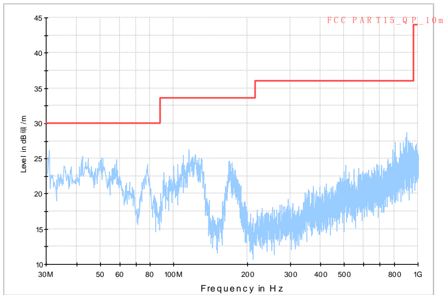
Normal RE_30M-1GHz_10m
