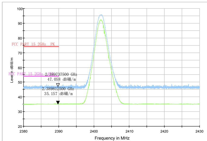
RE-BT-Power_2.38G-2.43GHz
