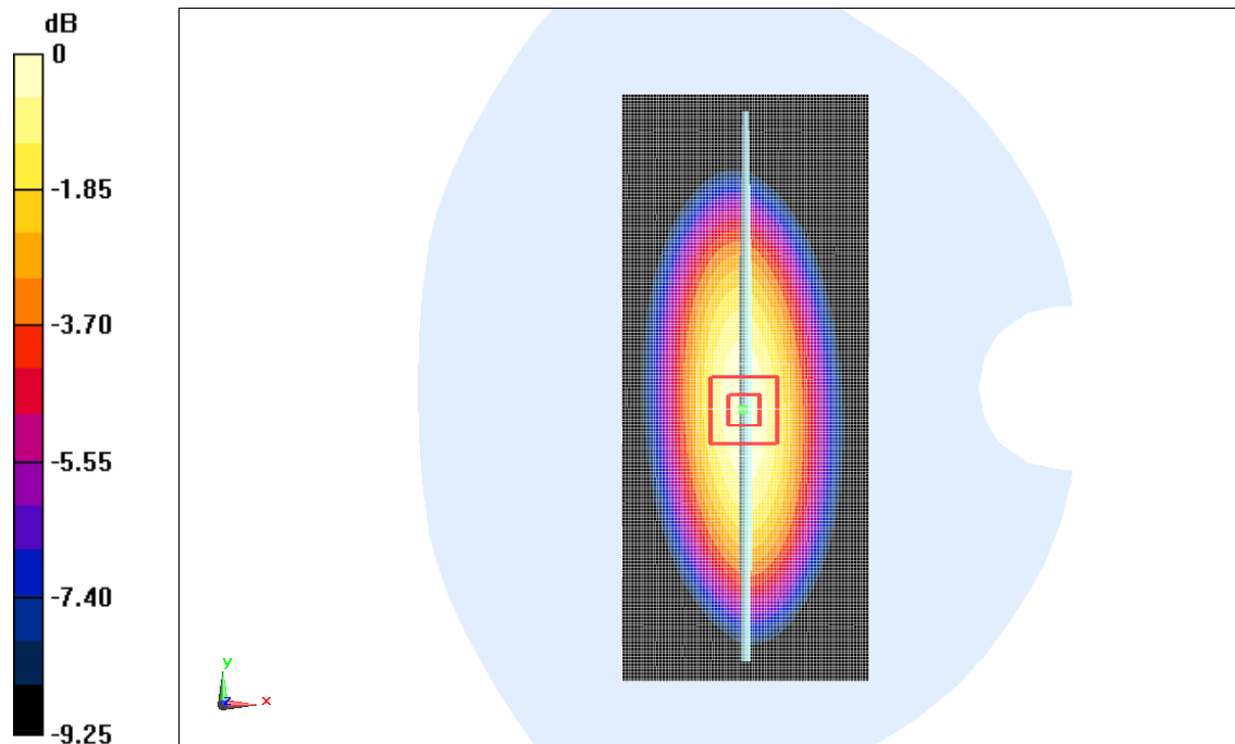
Fig.B.1 validation 750MHz 250mW
