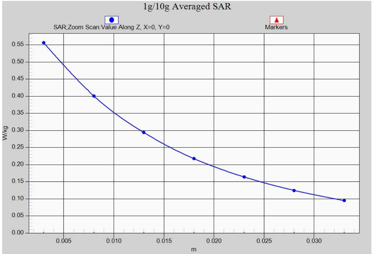
Fig. 6-1 Z-Scan at power reference point (LTE Band13)
