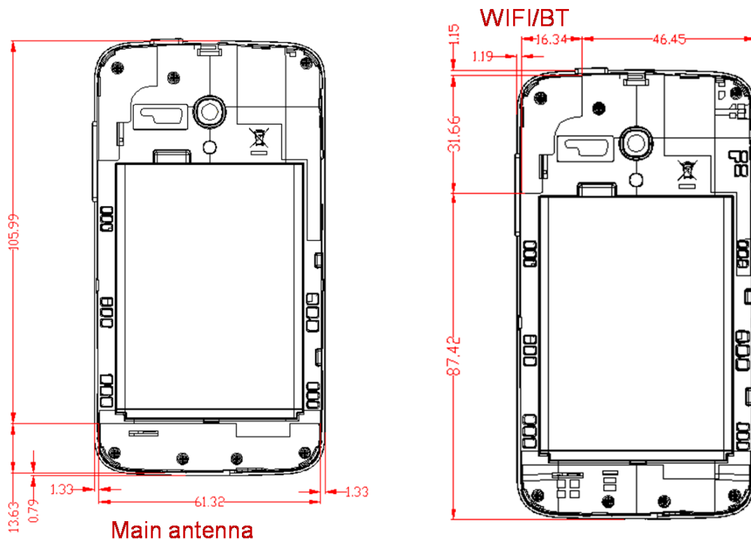
Picture 12.1 Antenna Locations
