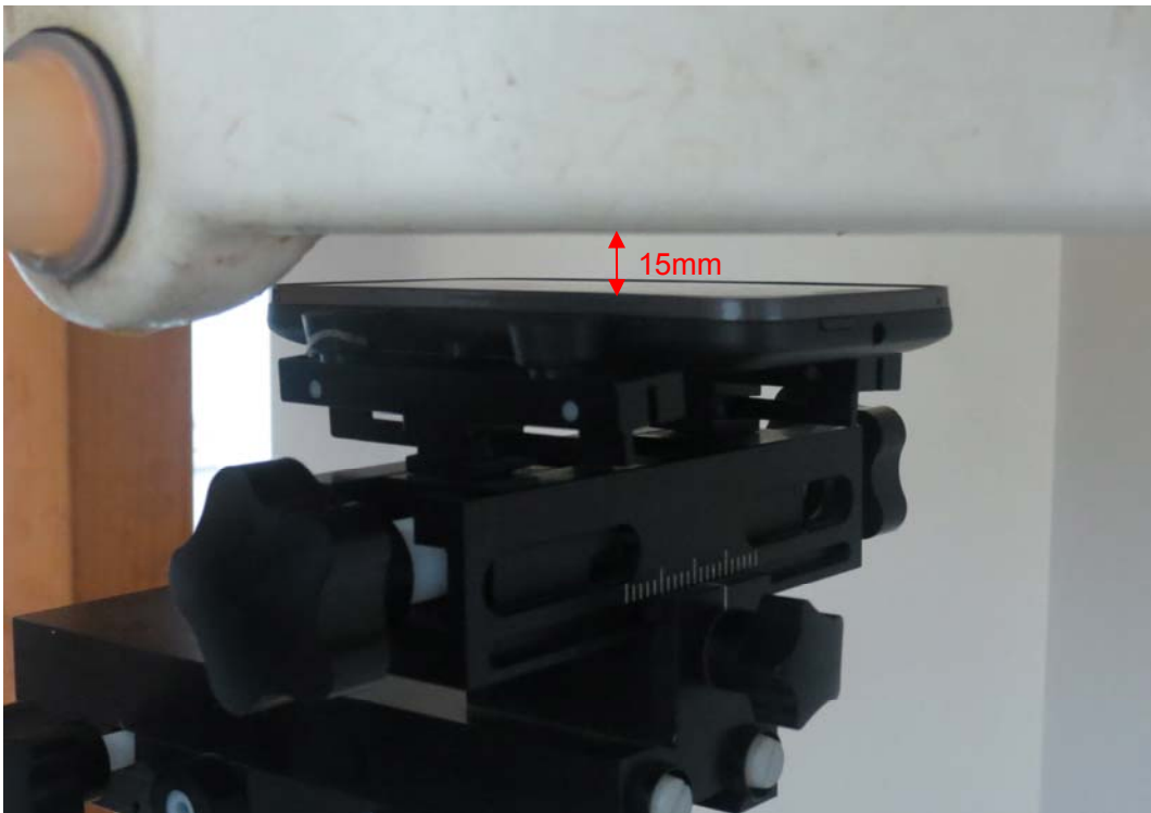
Picture 18: Front Side, the distance from handset to the bottom of the Phantom is 15mm
