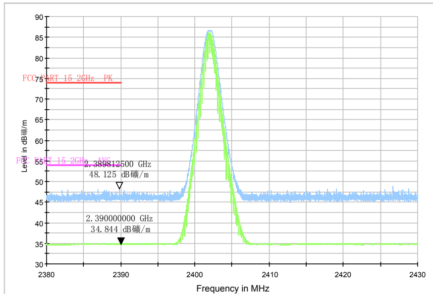
RE-BT-Power_2.38G-2.43GHz
