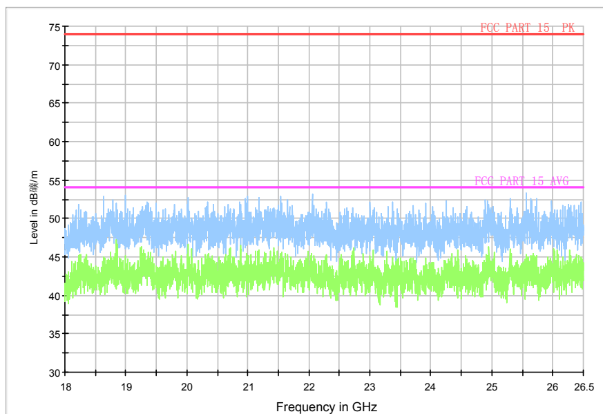
Normal RE_18G-26.5GHz
