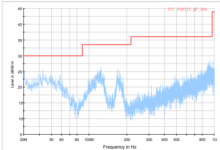
Normal RE_30M-1GHz_10m
