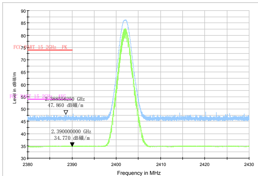
RE-BT-Power_2.38G-2.43GHz
