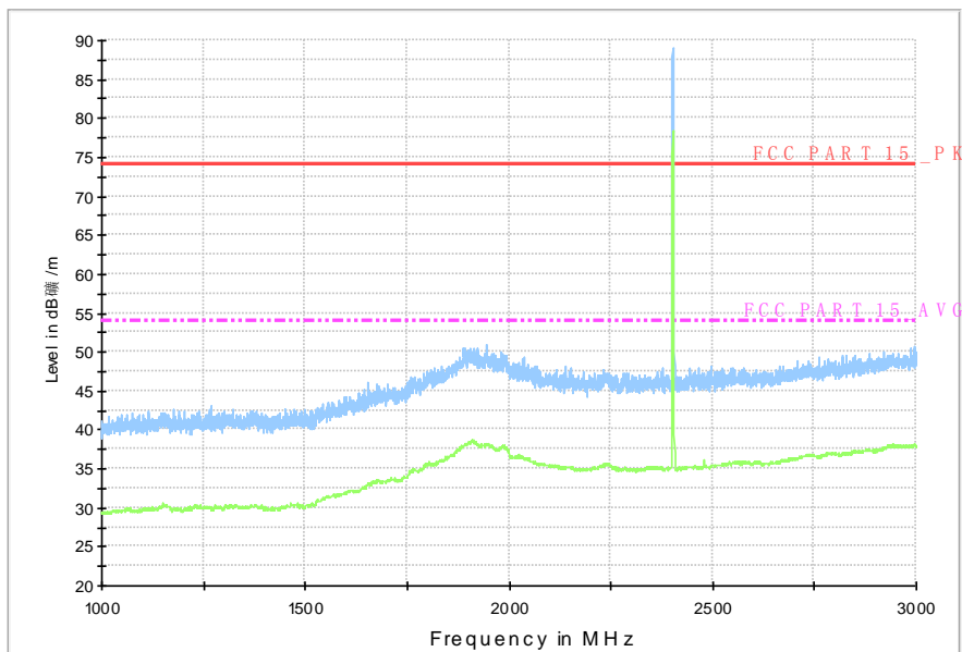
RE_BT_1G-3GHz
