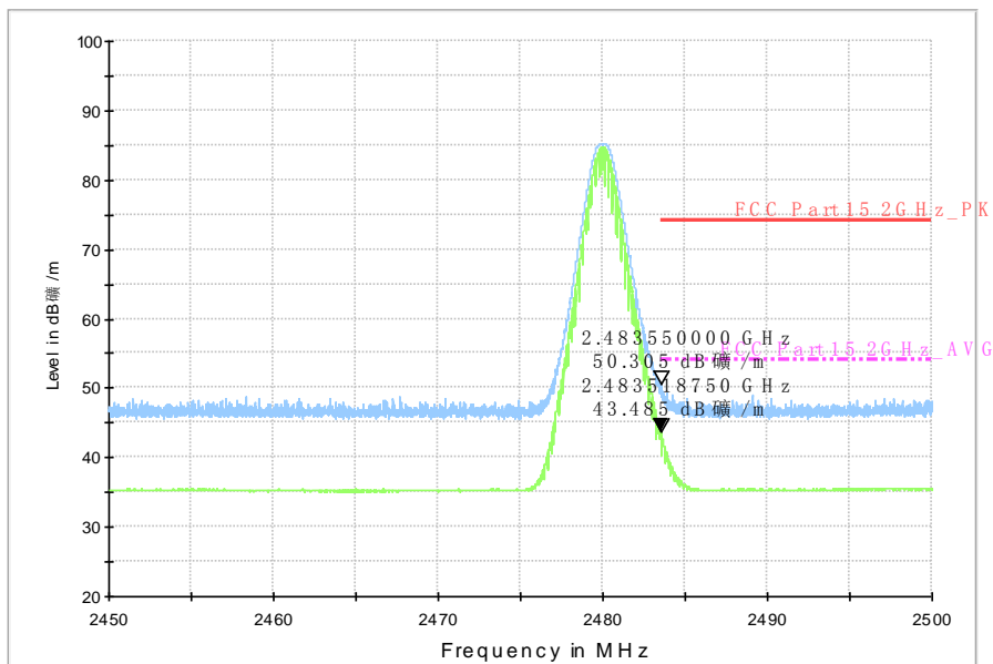
RE-BT-Power_2.45G-2.5GHz
