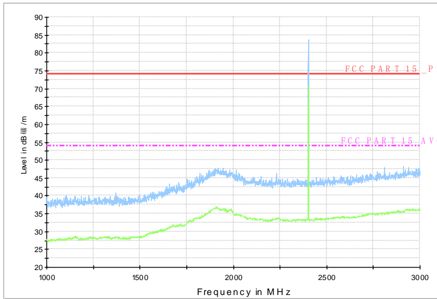
RE_W LAN_1G-3GHz
