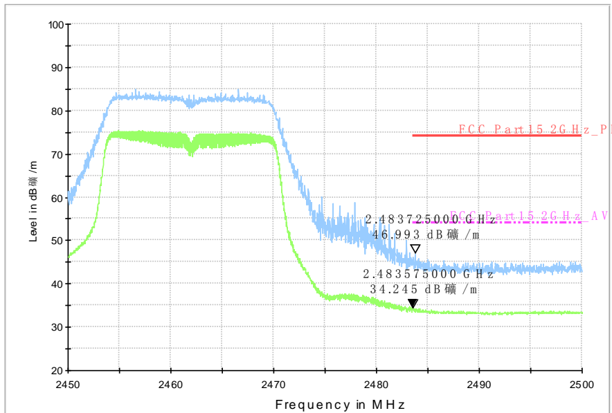
RE-Power_2.45G-2.5GHz
