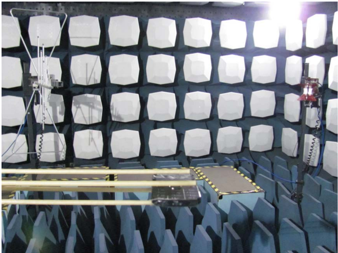
Radiated Spurious Emission Test Layout
