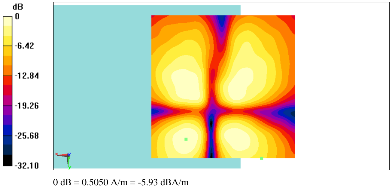
Fig B.1 T-Coil CDMA 835
