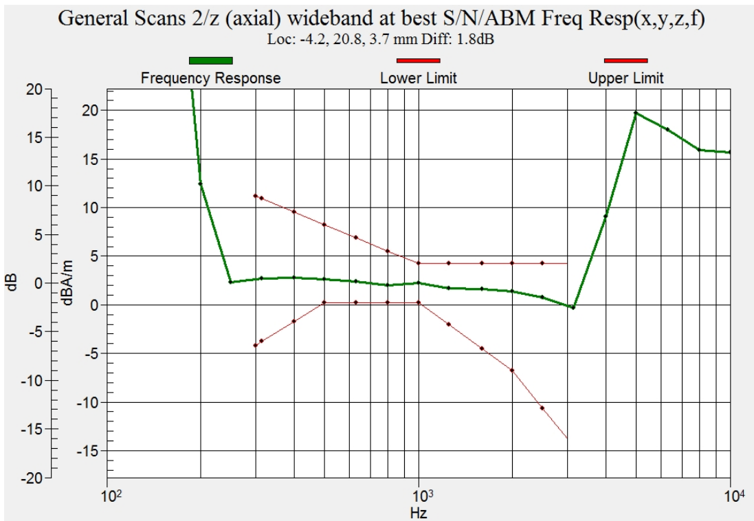
Figure C.2 Frequency Response of CDMA 1880
