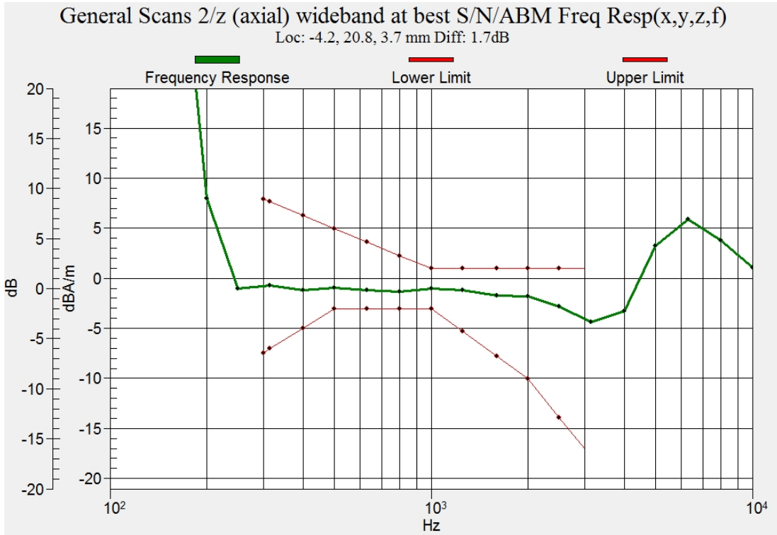
Figure C.1 Frequency Response of CDMA 835
