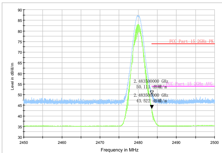
RE-BT-Power_2.45G-2.5GHz
