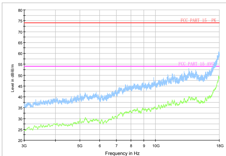
Normal RE_3G-18GHz
