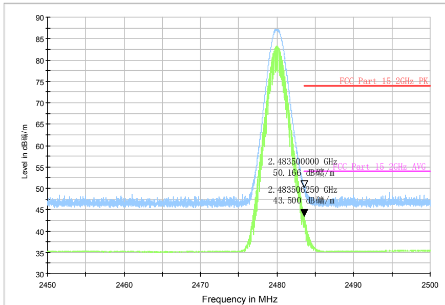
RE-BT-Power_2.45G-2.5GHz
