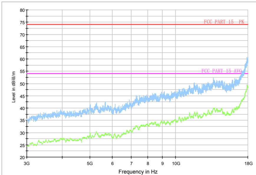
Normal RE_3G-18GHz
