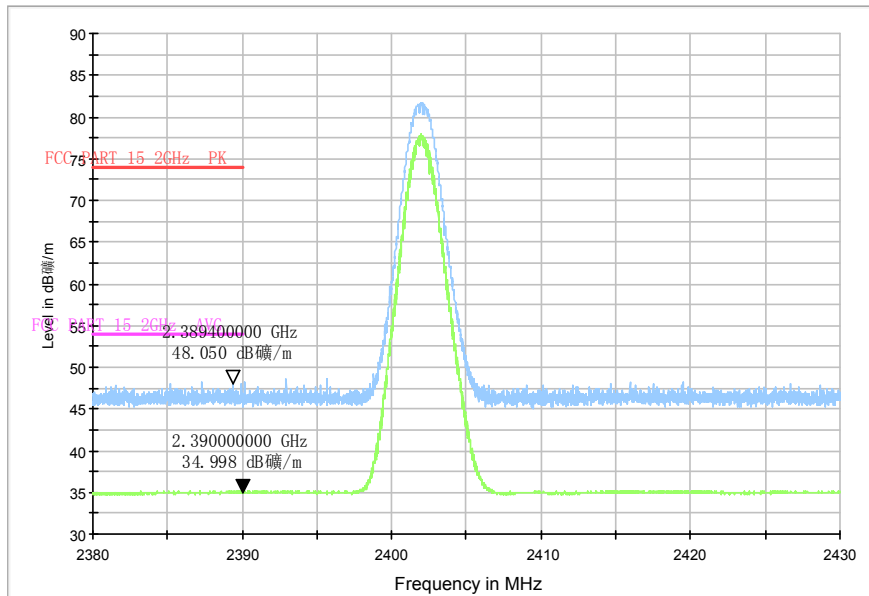
RE-BT-Power_2.38G-2.43GHz
