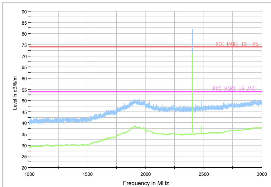
RE_BT_1G-3GHz
