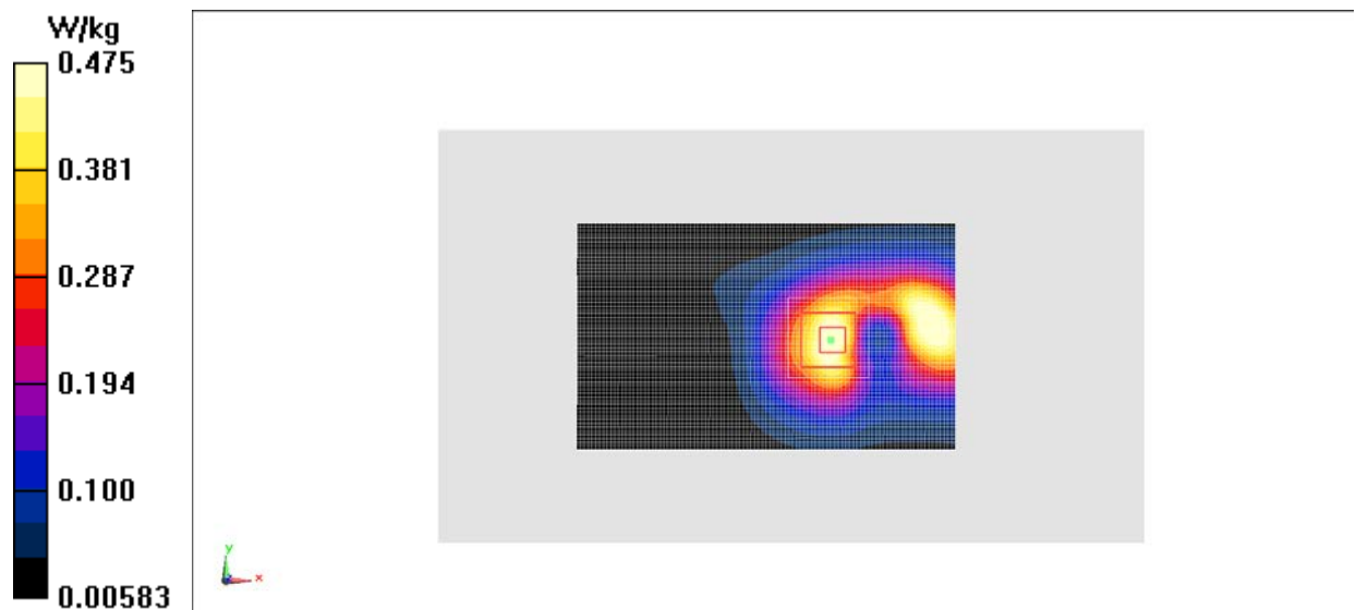
Fig.4 1900 MHz CH810
