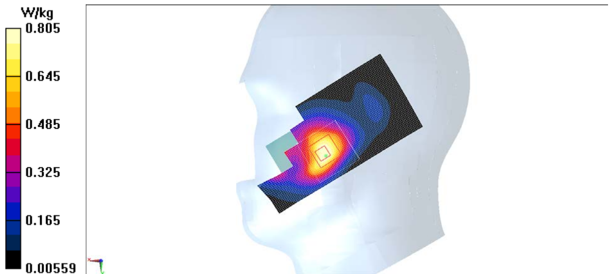
Fig.3 1900 MHz CH810
