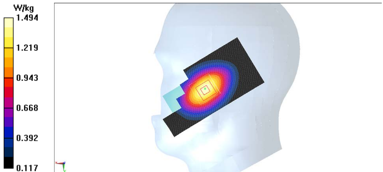
Fig.1 850MHz CH251
