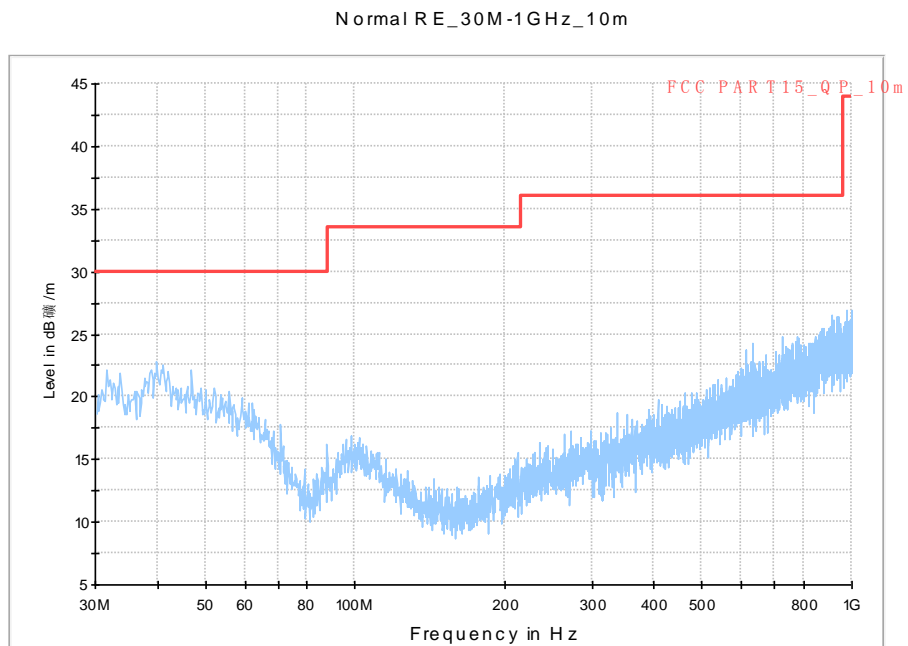
Fig.80. Radiated emission: 8DPSK, Channel 39, 30 MHz - 1 GHz
