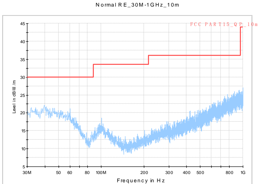
Fig.70. Radiated emission: \pi/4 DQPSK, Channel 39, 30 MHz - 1 GHz
