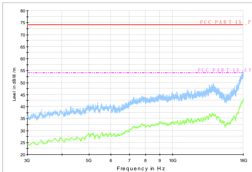
Normal RE_3G-18GHz
