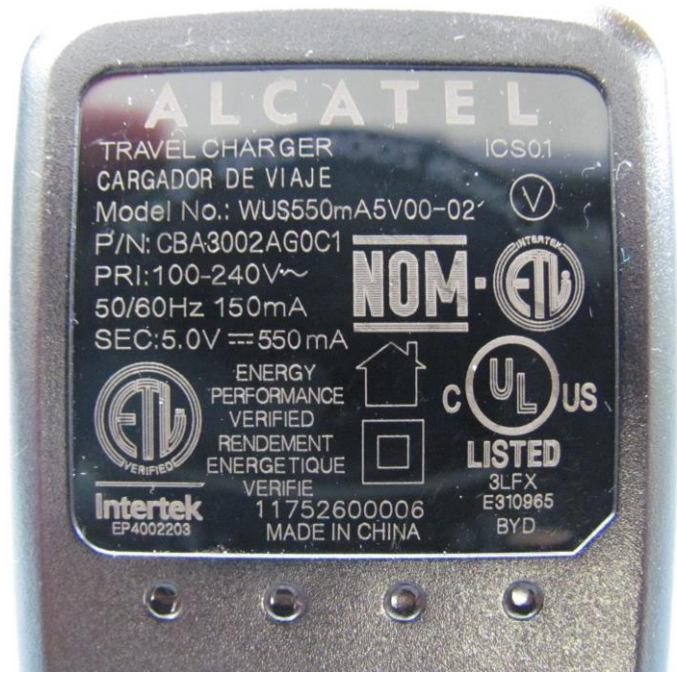
Charger
