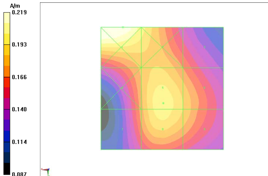
Fig B.15 HAC RF H-Field GSM 1900 Low
