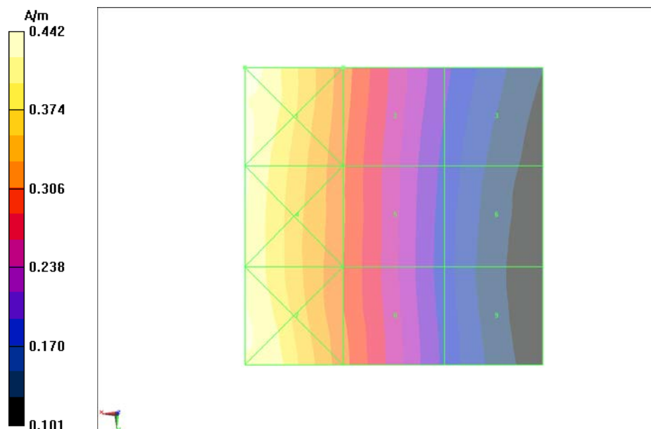
Fig B.10 HAC RF H-Field GSM 850 High
