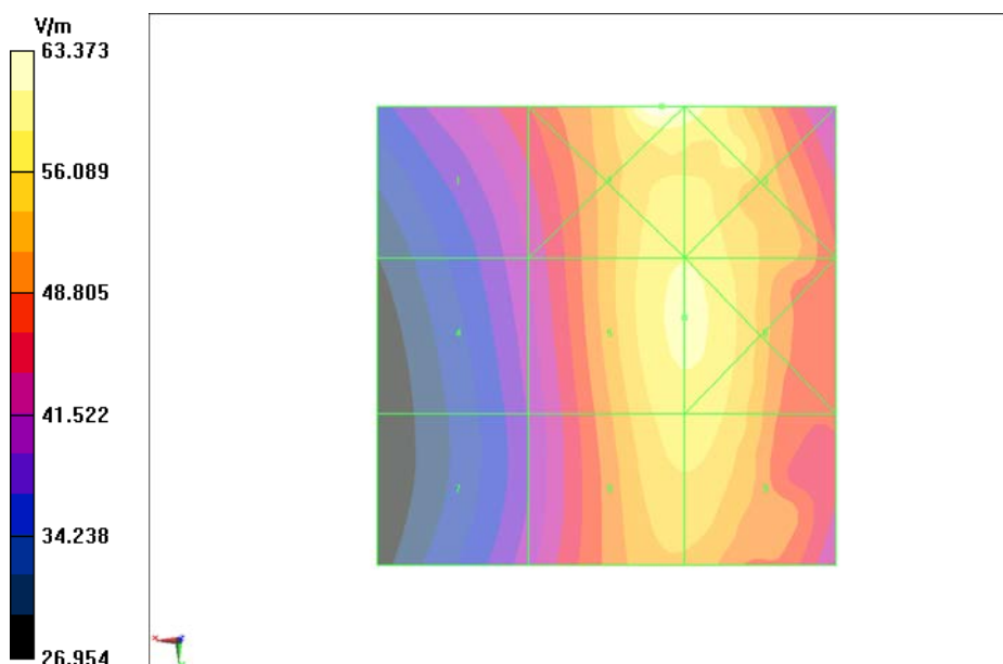
Fig B.7 HAC RF E-Field WCDMA 850 High
