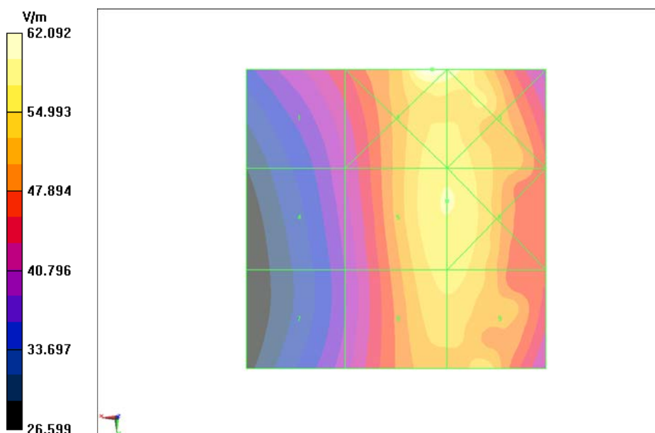
Fig B.8 HAC RF E-Field WCDMA 850 Middle
