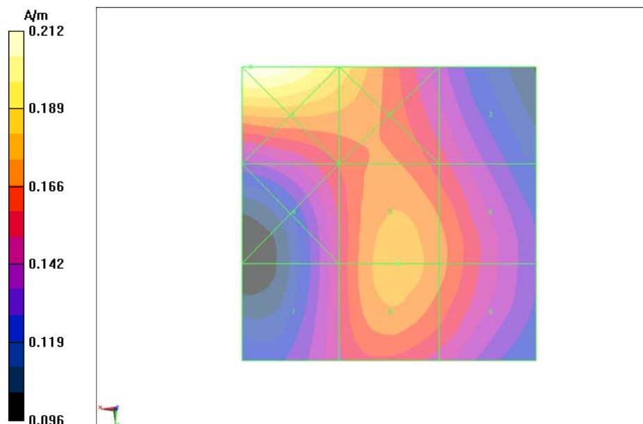
Fig B.14 HAC RF H-Field GSM 1900 Middle
