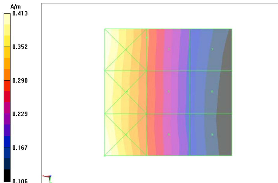
Fig B.11 HAC RF H-Field GSM 850 Middle
