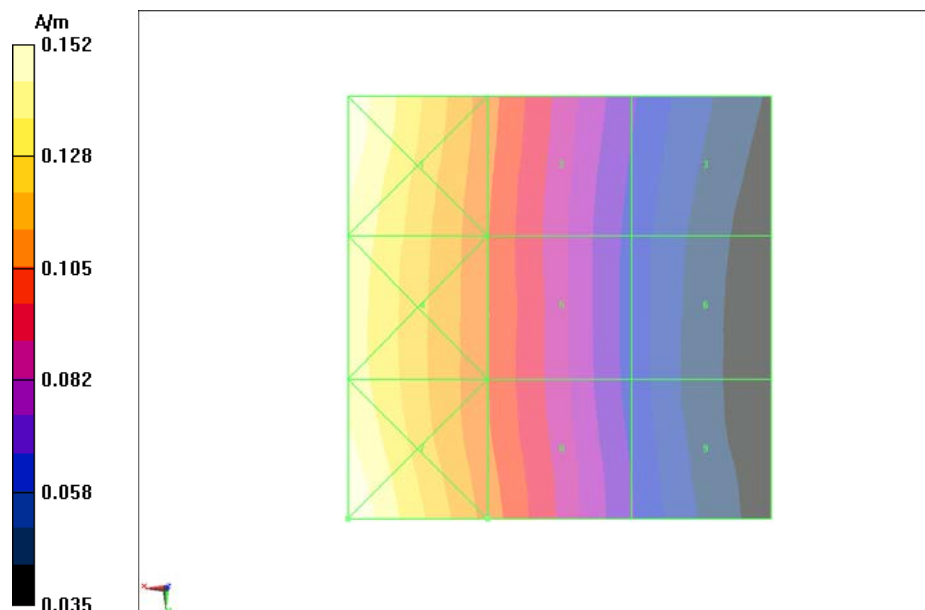
Fig B.17 HAC RF H-Field WCDMA 850 Middle
