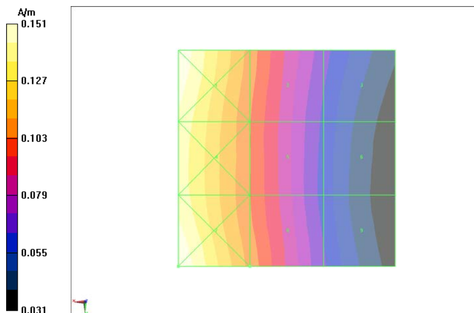
Fig B.16 HAC RF H-Field WCDMA 850 High
