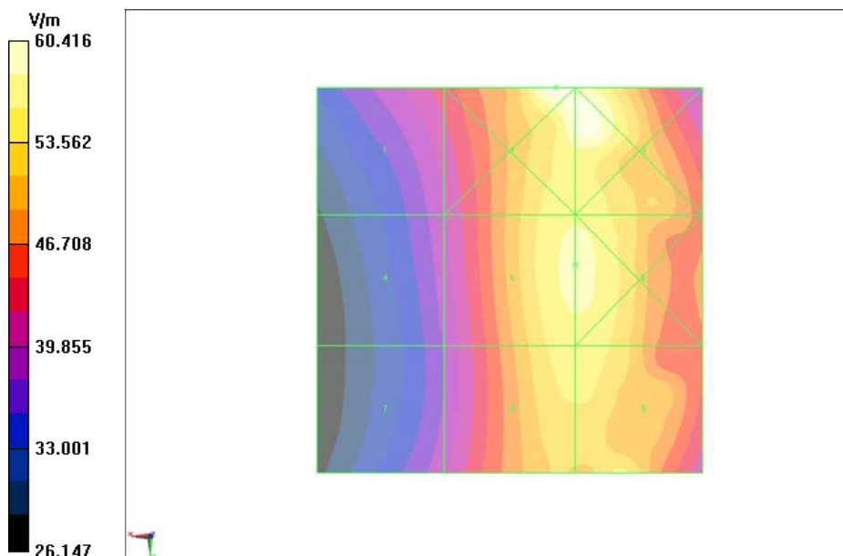
Fig B.9 HAC RF E-Field WCDMA 850 Low
