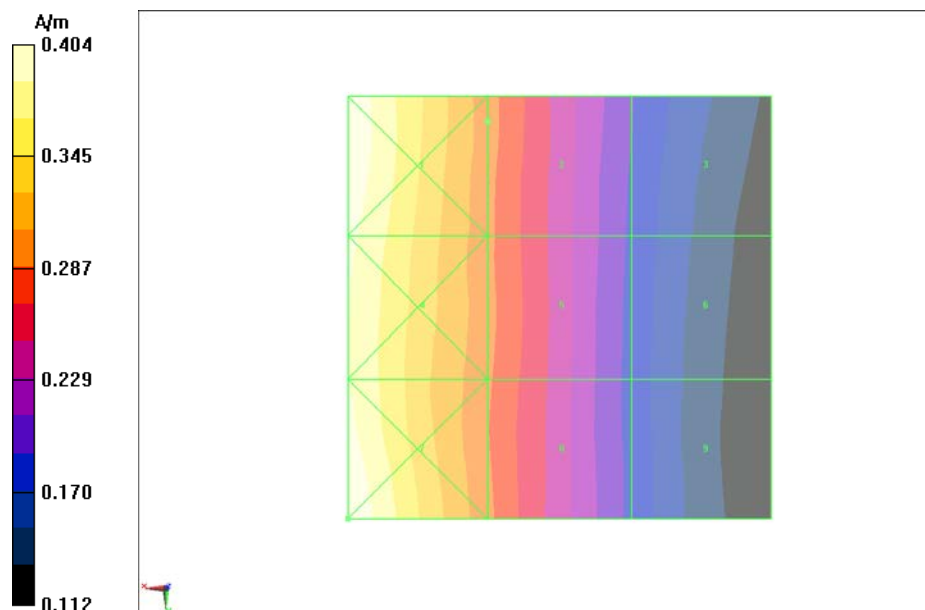
Fig B.12 HAC RF H-Field GSM 850 Low
