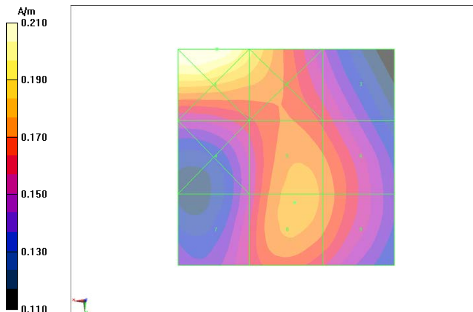
Fig B.13 HAC RF H-Field GSM 1900 High
