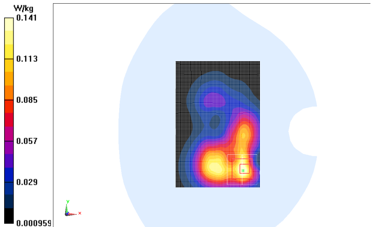
Fig.8 2450 MHz CH11
