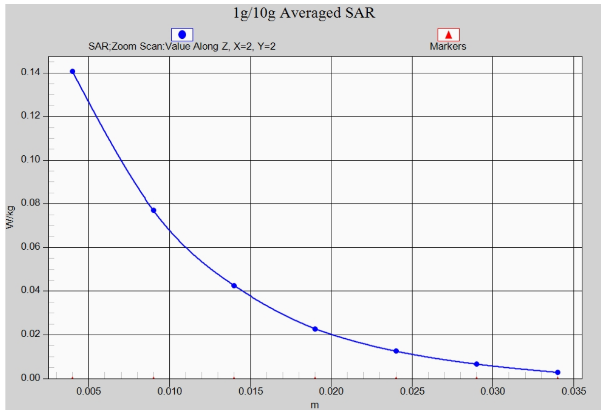
Fig. 8-1 Z-Scan at power reference point (2450 MHz CH11)
