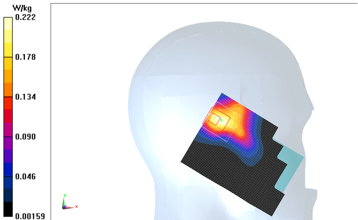
Fig.7 2450 MHz CH11
