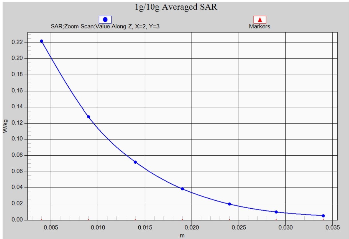
Fig. 7-1 Z-Scan at power reference point (2450 MHz CH11)
