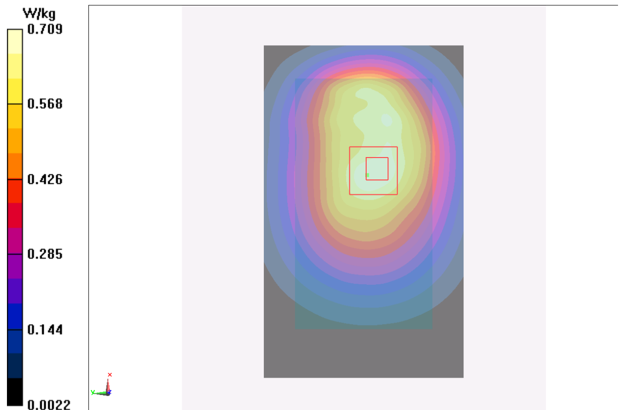
Fig.2 850 MHz CH128
