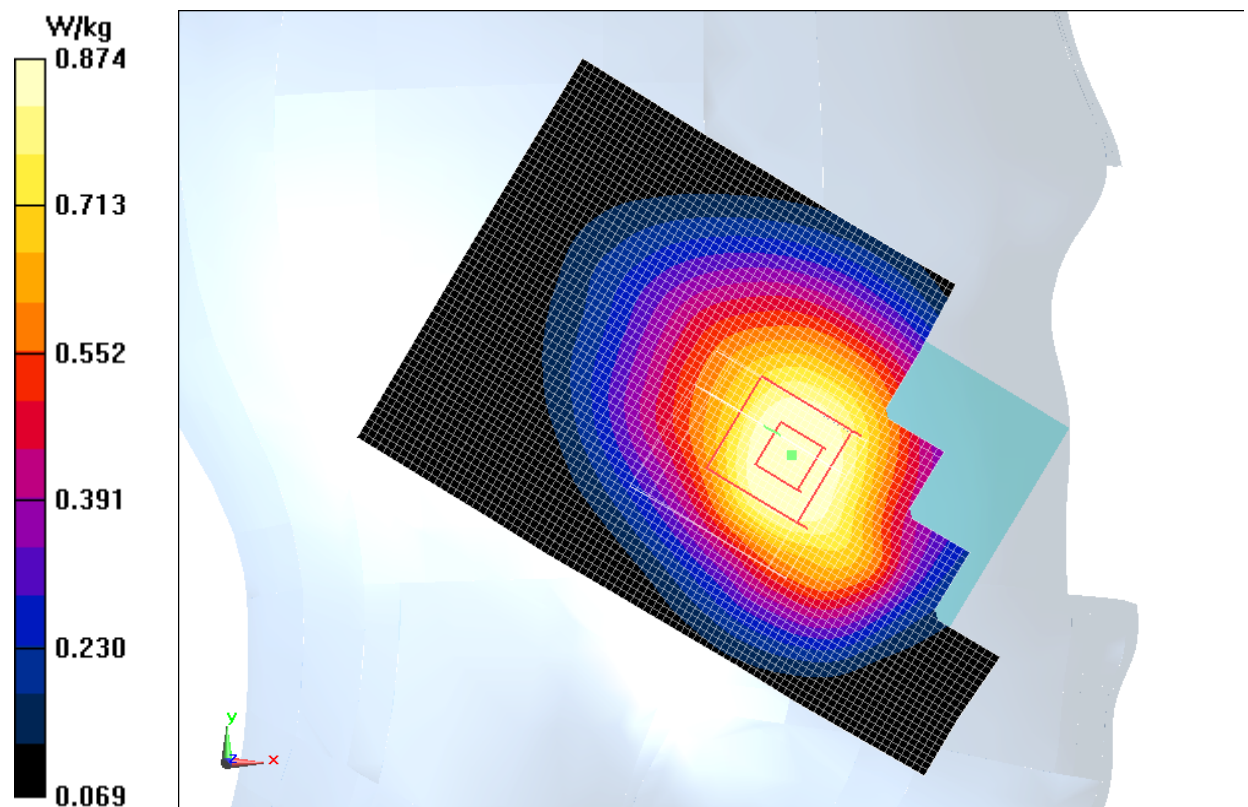
Fig.5 WCDMA 850 CH4132
