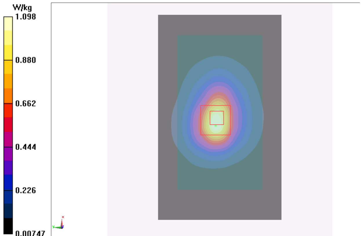
Fig.4 1900 MHz CH810
