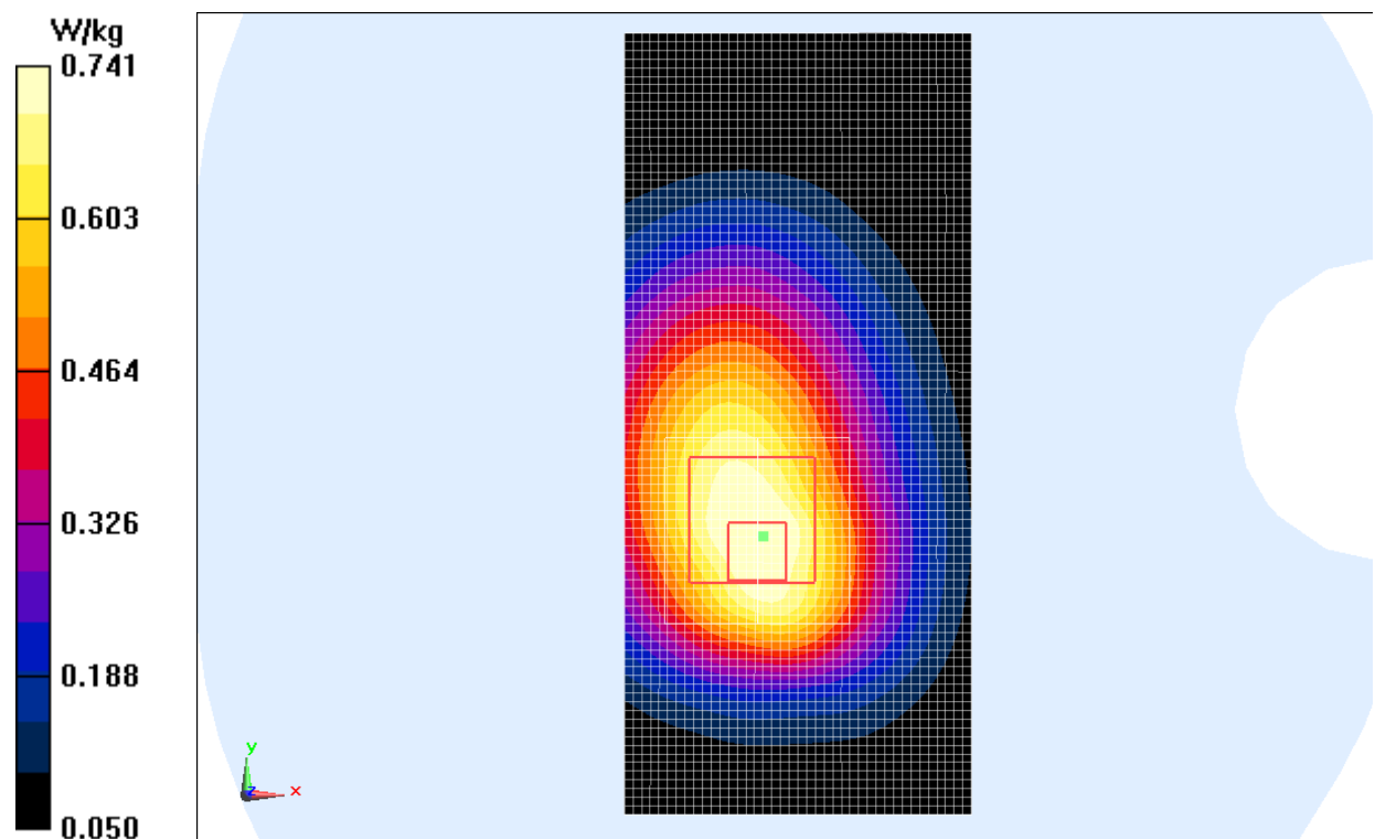
Fig.6 WCDMA 850 CH4132
