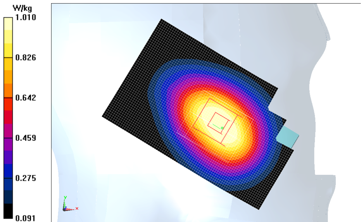
Fig.5 WCDMA 850 CH4132
