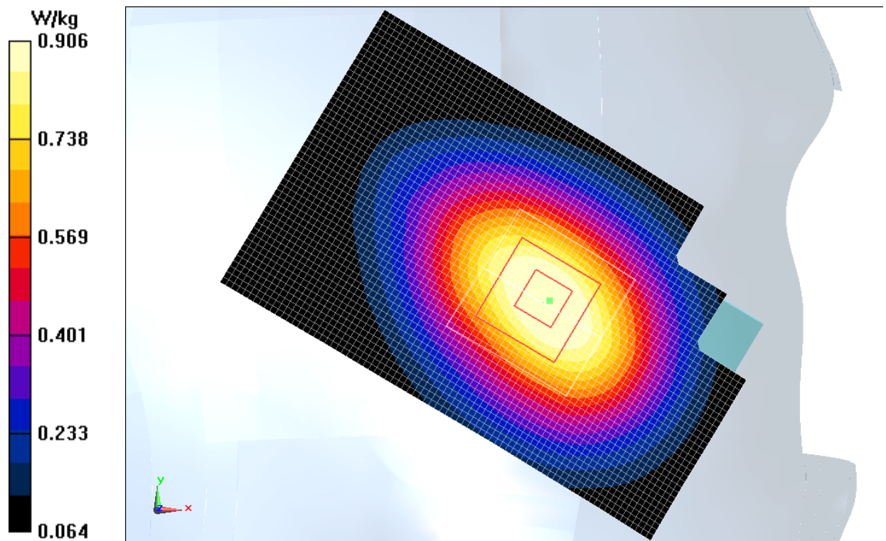
Fig.1 850MHz CH251
