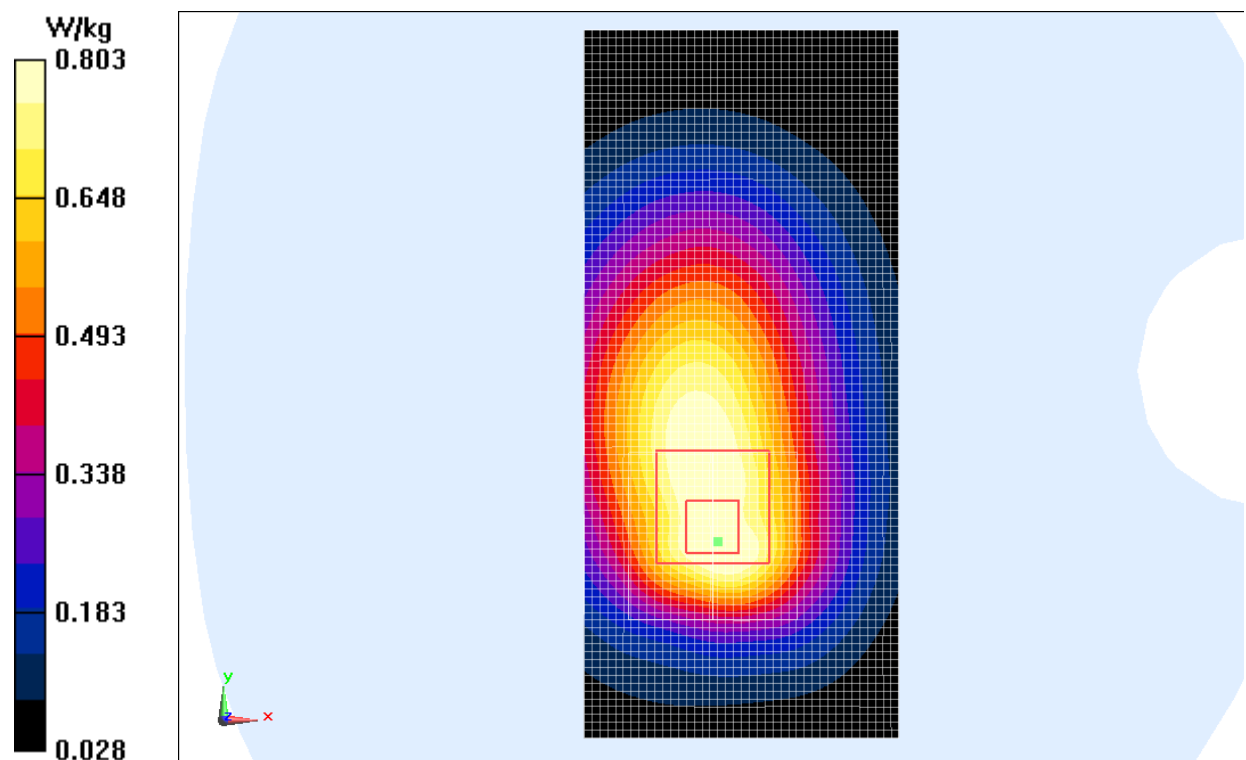
Fig.2 850 MHz CH190
