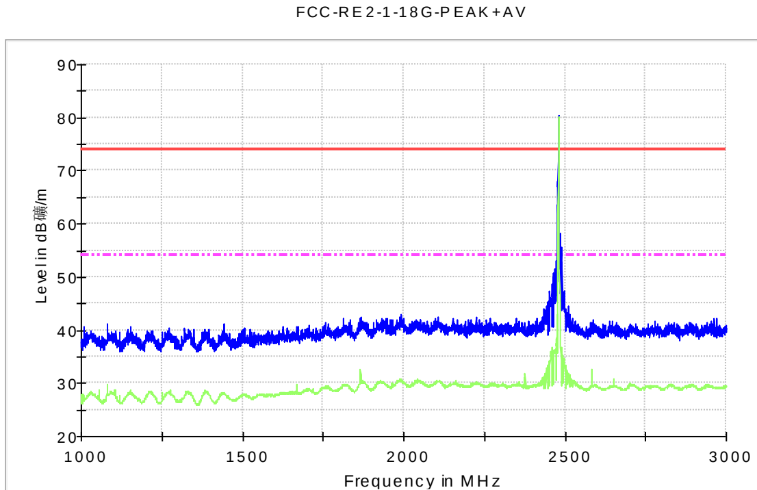
Fig.54. Radiated emission: \pi/4 DQPSK, Channel 78, 1 GHz - 3 GHz
