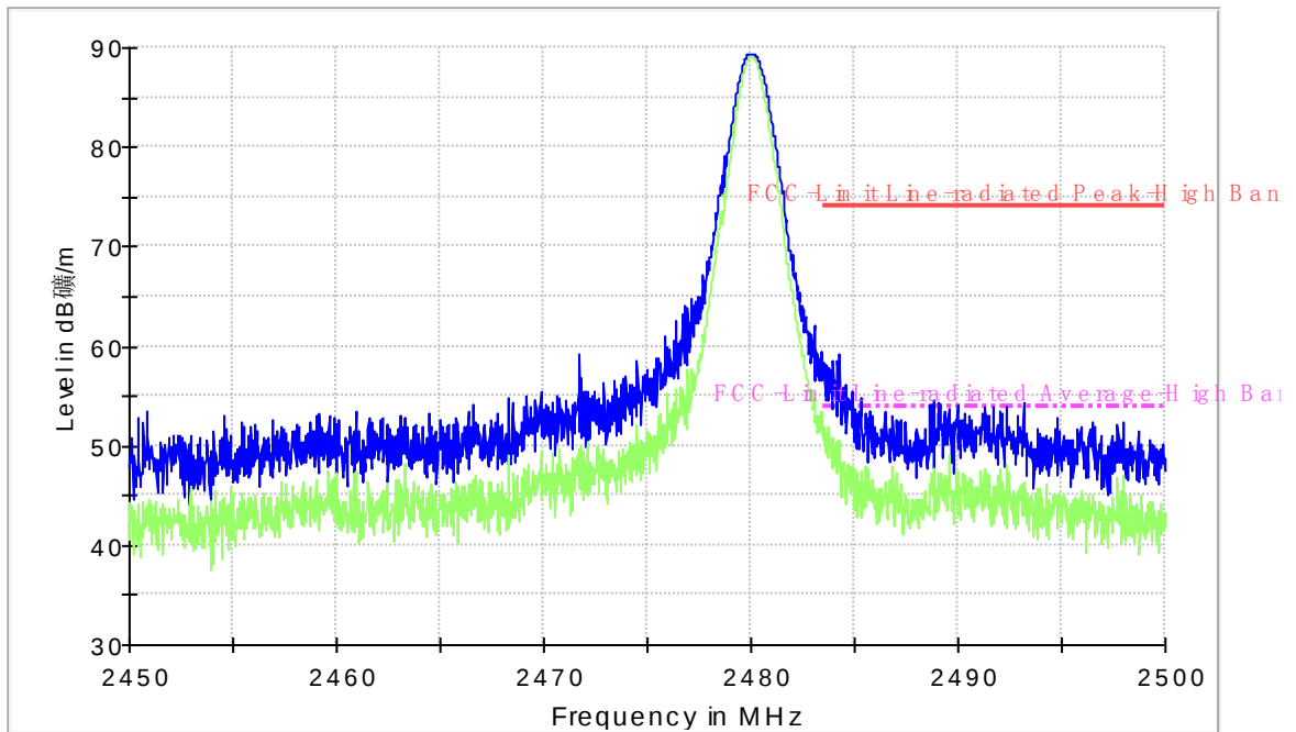
FCC-RE2-BAND Edge-High Band
