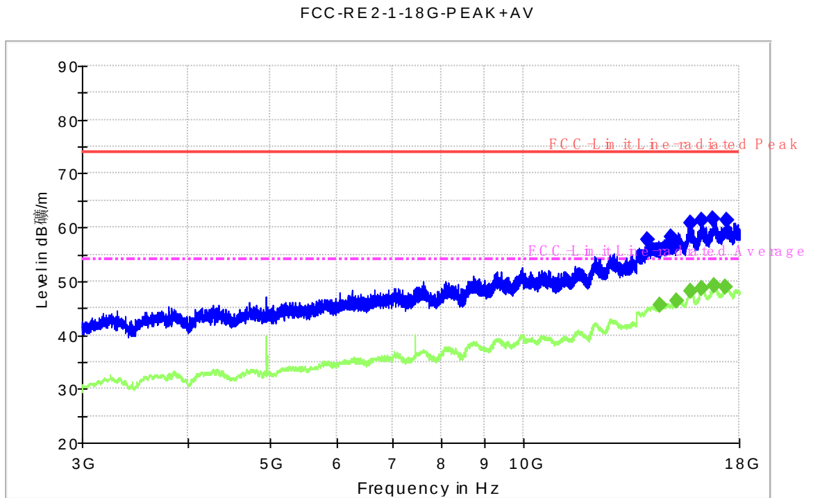
Fig.55. Radiated emission: \pi/4 DQPSK, Channel 78, 3 GHz - 18 GHz
