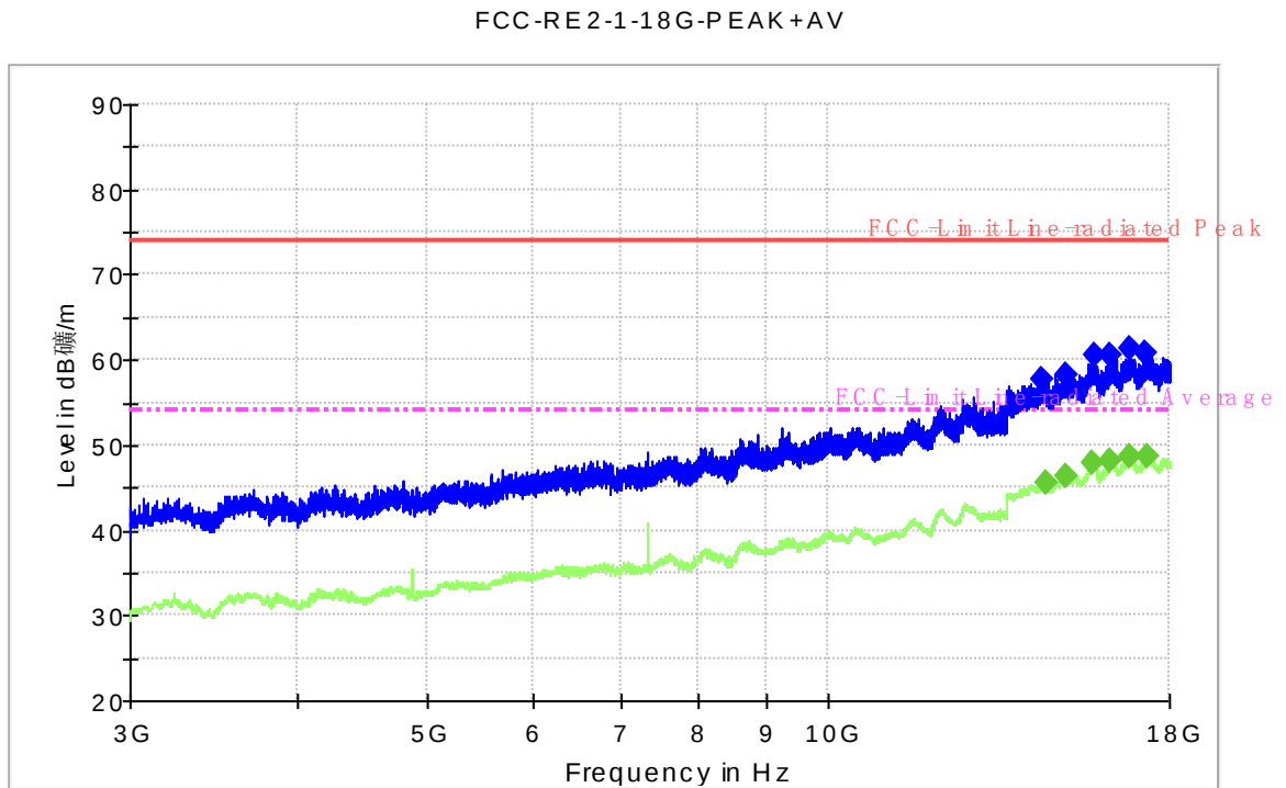
Fig.43. Radiated emission: GFSK, Channel 39, 3 GHz - 18 GHz
