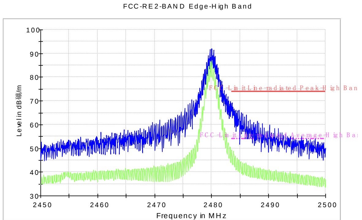
Fig.57. Radiated emission (Power): \pi/4 DQPSK, high channel
