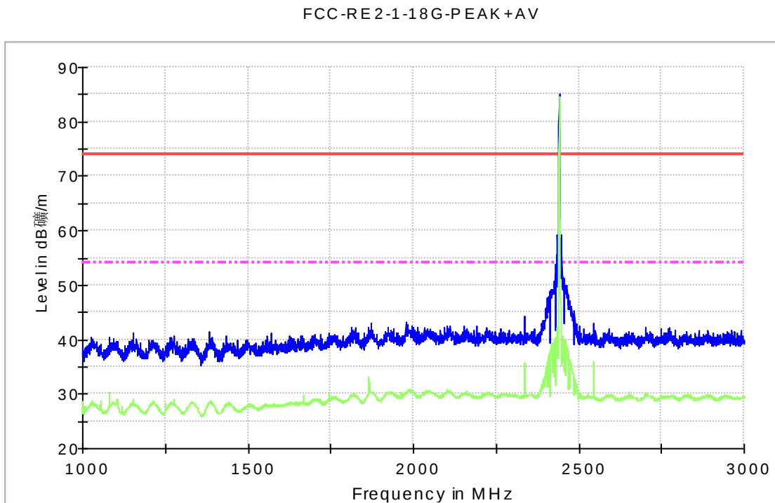
Fig.42. Radiated emission: GFSK, Channel 39, 1 GHz - 3 GHz
