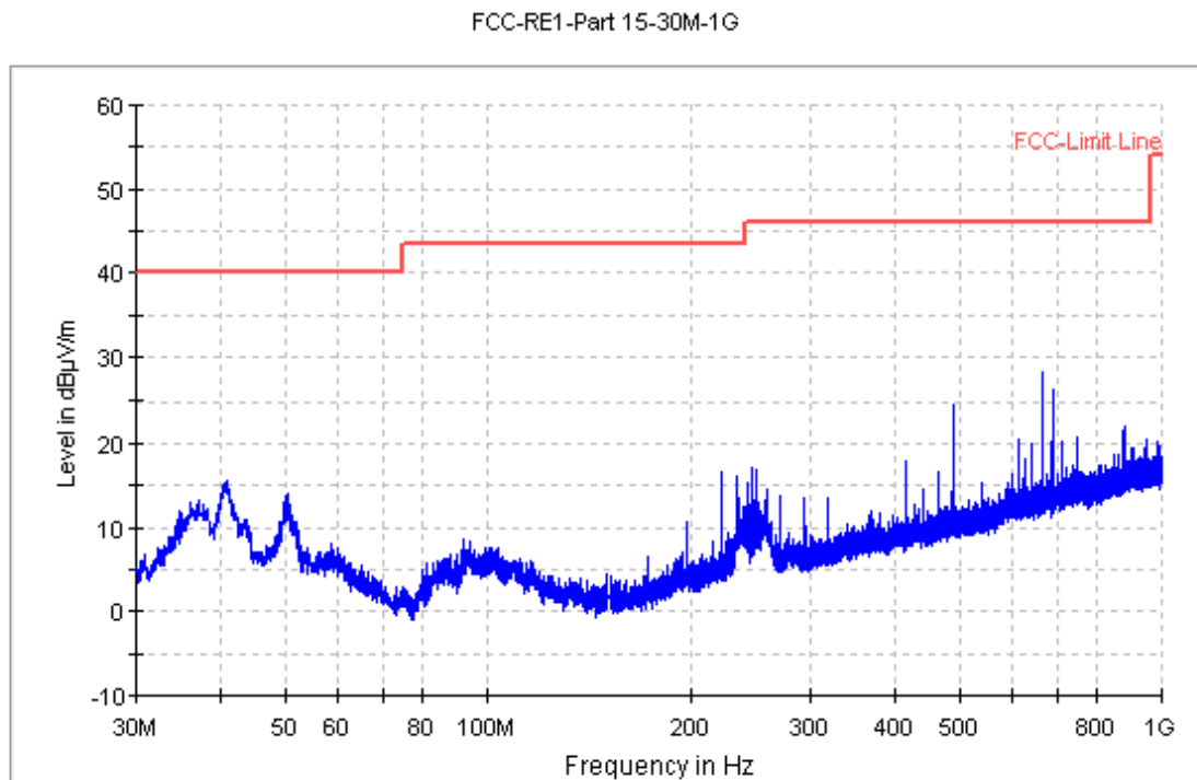
Fig.41. Radiated emission: GFSK, Channel 39, 30 MHz - 1 GHz
