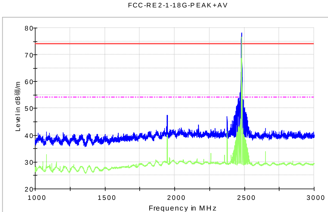
Fig.44. Radiated emission: GFSK, Channel 78, 1 GHz - 3 GHz
