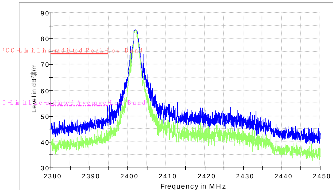
FCC-RE2-BAND Edge-Low Band
