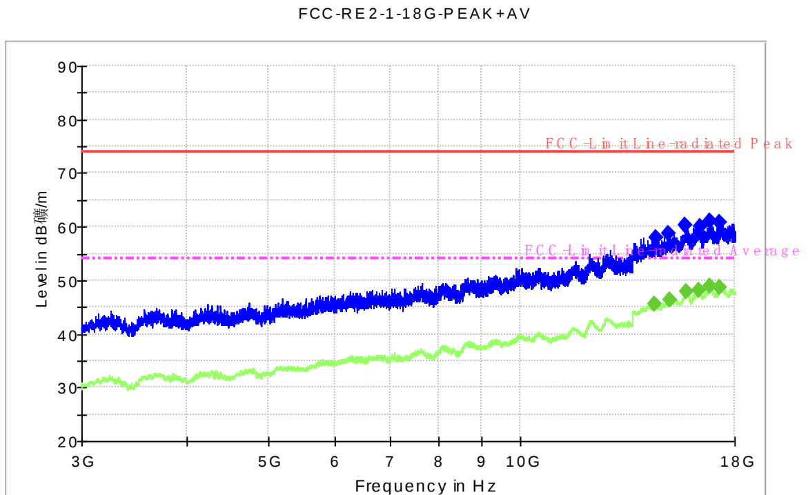
Fig.50. Radiated emission: \pi/4 DQPSK, Channel 0, 3 GHz - 18 GHz
