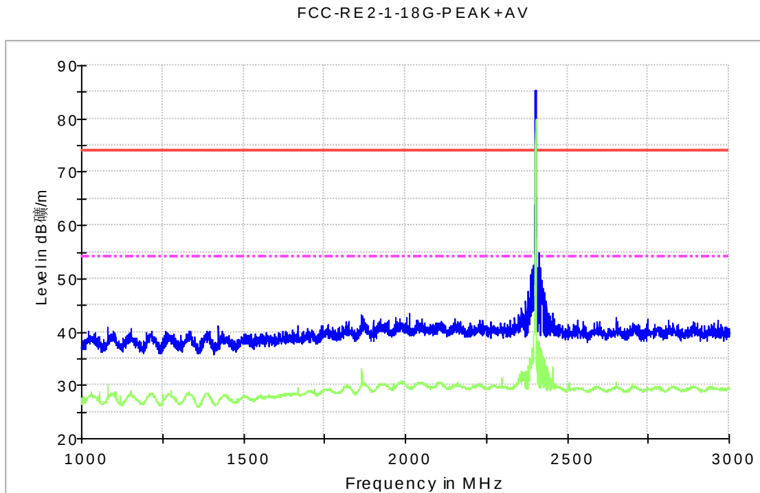
Fig.49. Radiated emission: \pi/4 DQPSK, Channel 0, 1 GHz - 3 GHz
