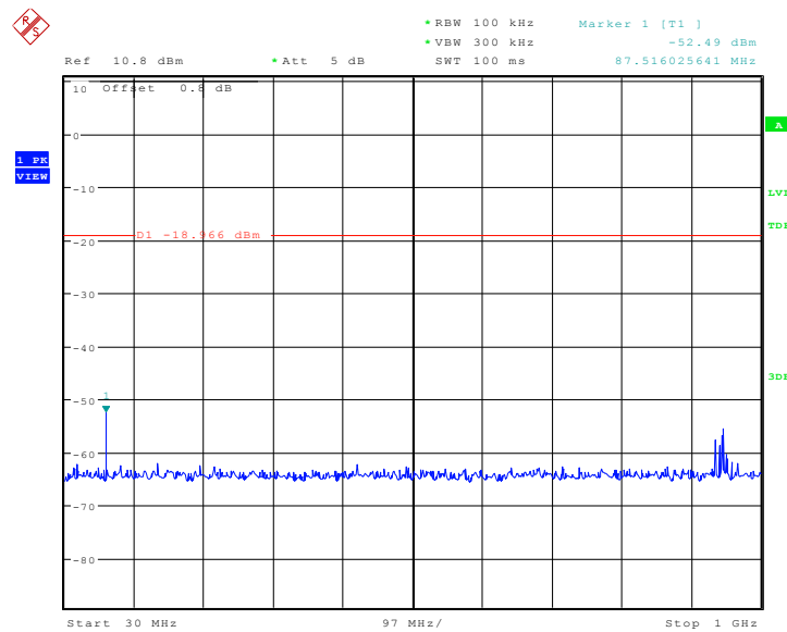
Fig.9. Conducted spurious emission: GFSK, Channel 0,2402MHz
