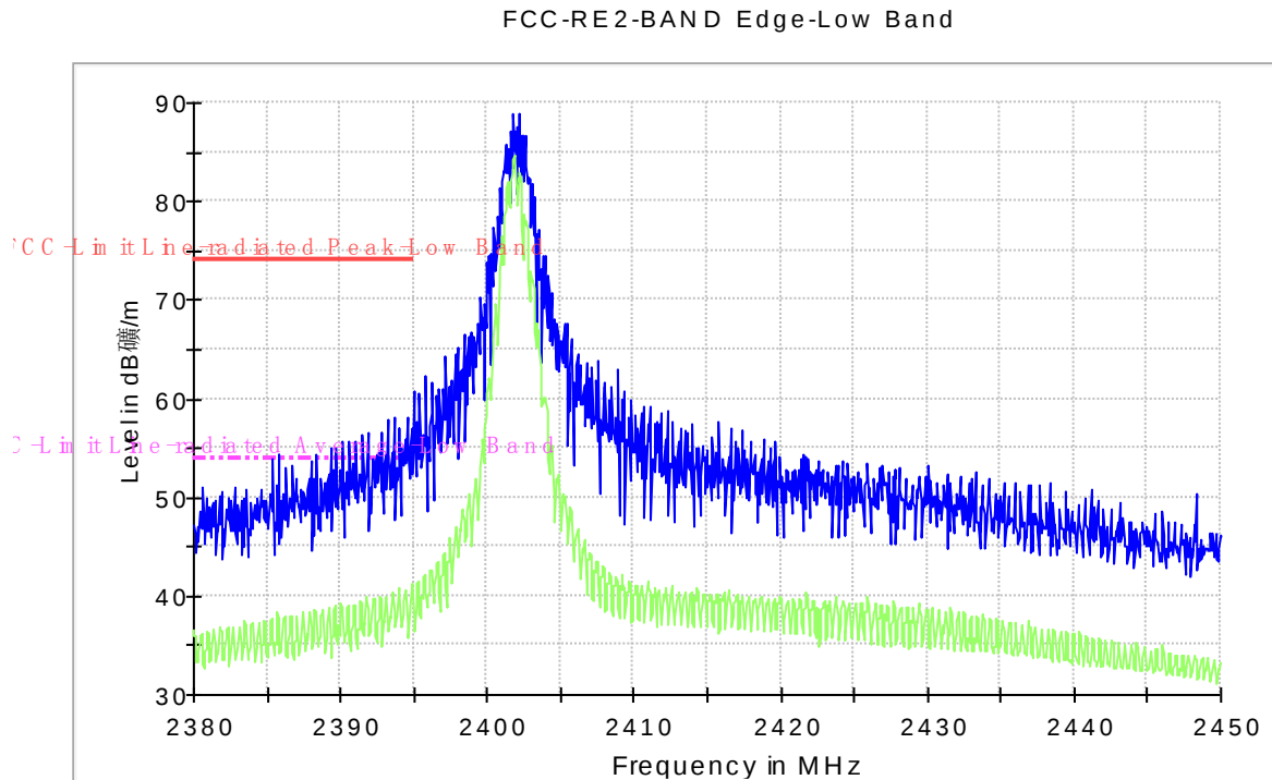
Fig.56. Radiated emission (Power): \pi/4 DQPSK, low channel
