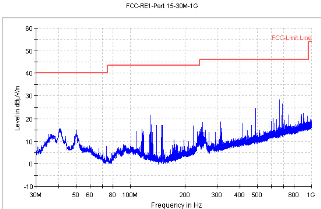
Fig.51. Radiated emission: \pi/4 DQPSK, Channel 39, 30 MHz - 1 GHz
