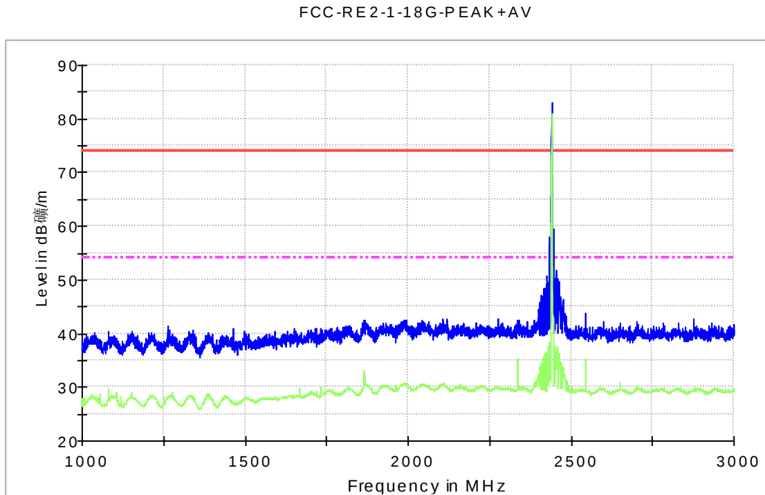
Fig.52. Radiated emission: \pi/4 DQPSK, Channel 39, 1 GHz - 3 GHz
