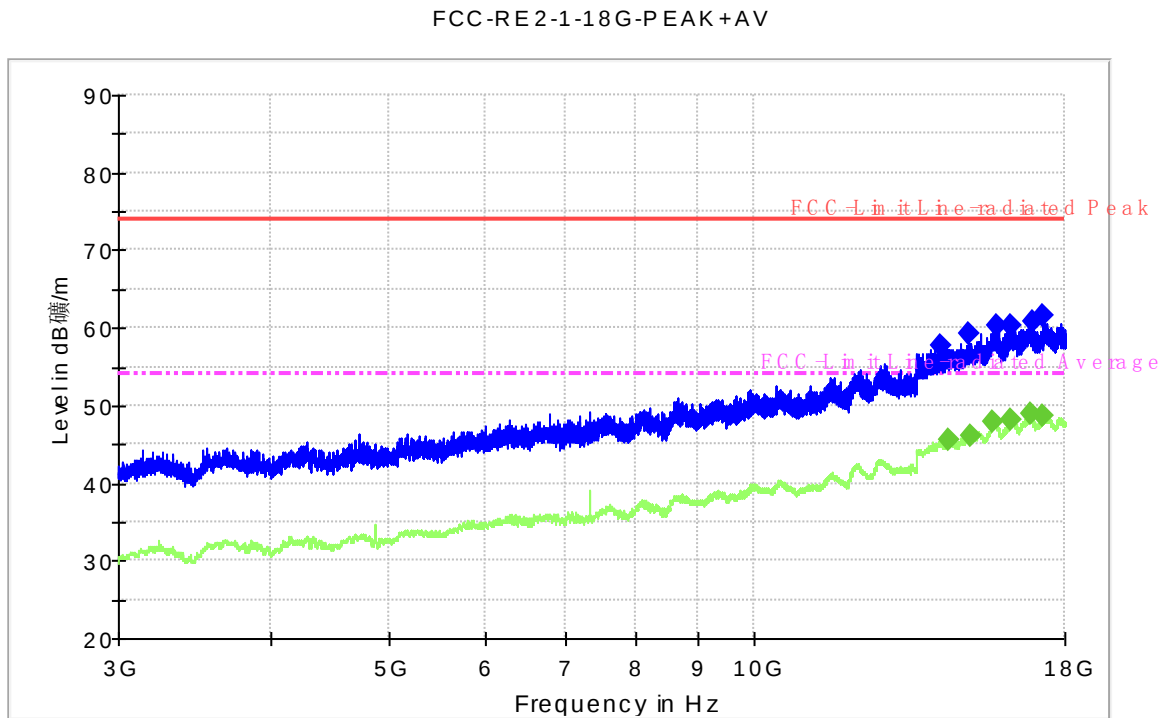
Fig.53. Radiated emission: \pi/4 DQPSK, Channel 39, 3 GHz - 18 GHz
