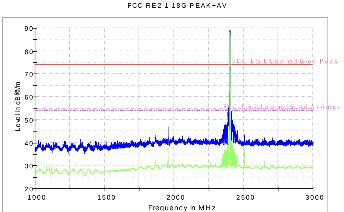
Fig.39. Radiated emission: GFSK, Channel 0, 1 GHz - 3 GHz
