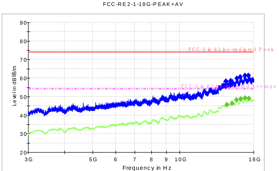
Fig.40. Radiated emission: GFSK, Channel 0, 3 GHz - 18 GHz
