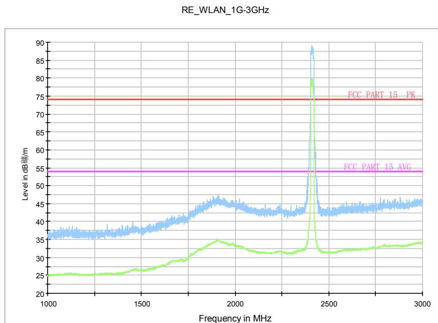
Fig.A.6.2.32 Radiated Spurious Emission (802.11n-RT20, Ch1, 1 GHz-3 GHz)
