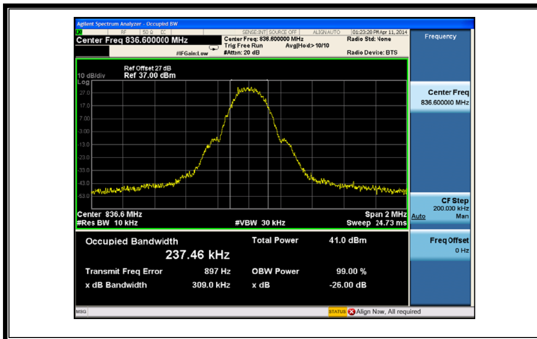
(Plot B1: GSM 850MHz Channel = 190)
