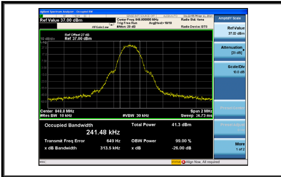
(Plot C1: GSM 850MHz Channel = 251)
