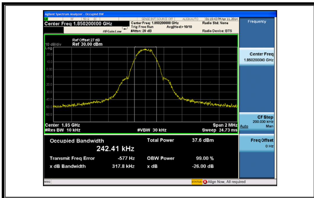
(Plot D1: GSM 1900MHz Channel = 512)
