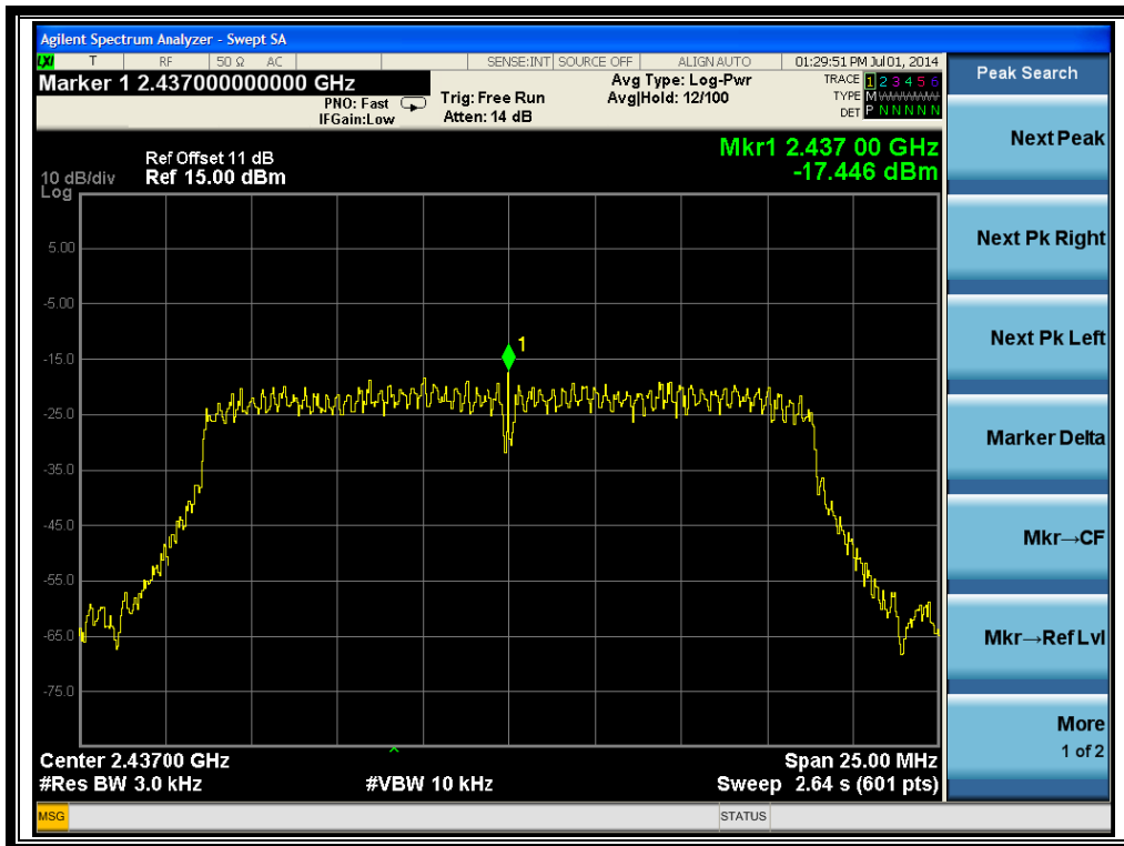
(Channel = 6 @ 802.11n-20MHz)
