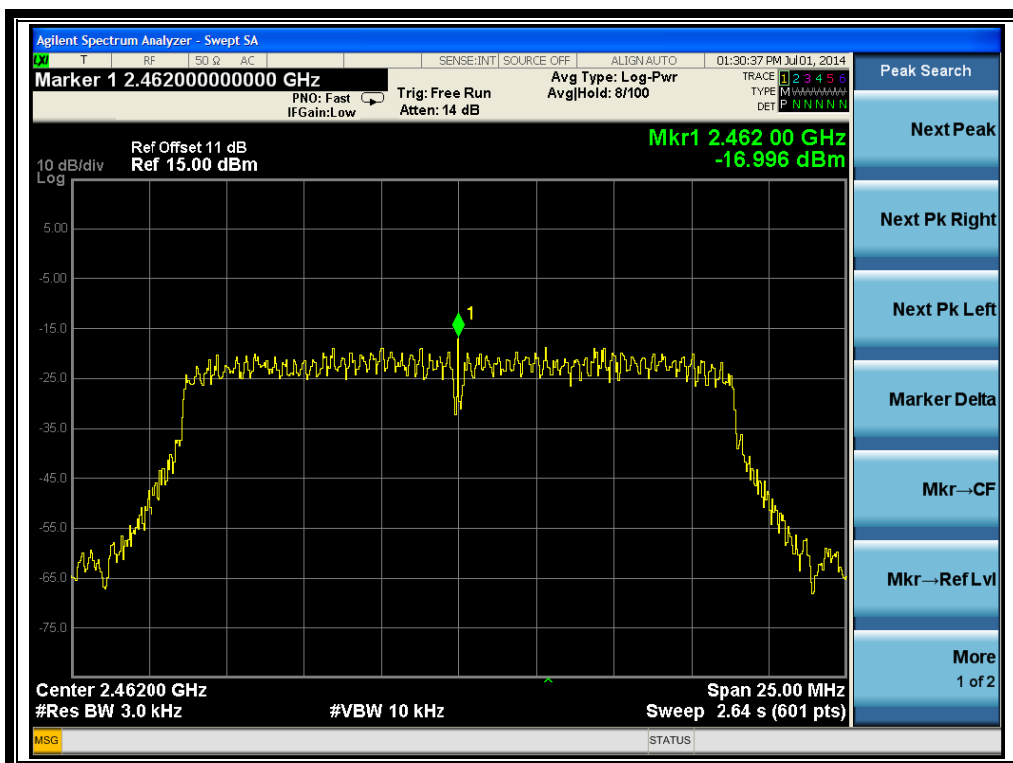
(Channel = 11 @ 802.11n-20MHz)
