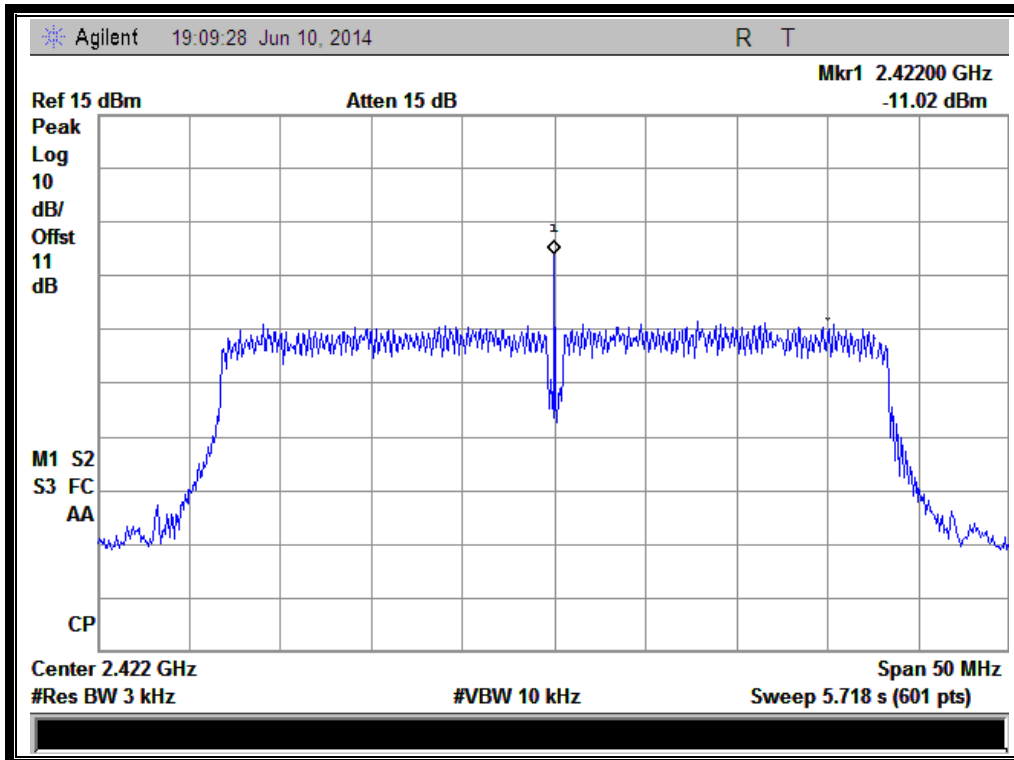
(Channel = 3 @ 802.11n-40MHz)
