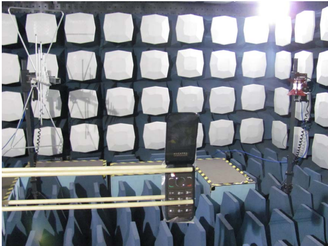
Pic F-2 Radiated Spurious Emission Test Layout
