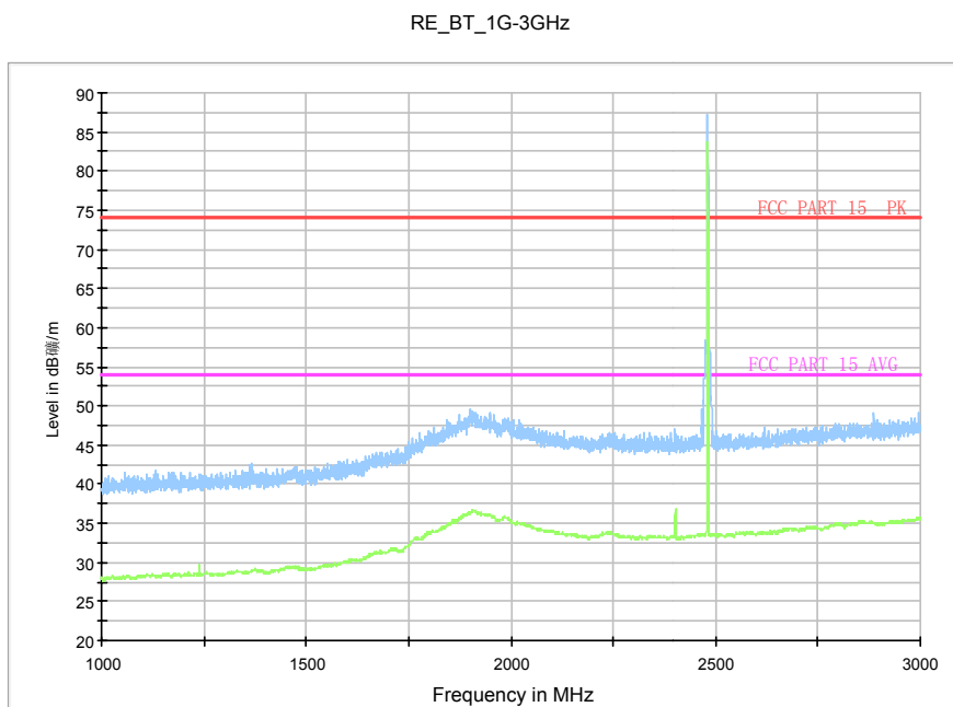
Fig.83. Radiated emission: 8DPSK, Channel 78, 1 GHz - 3 GHz
