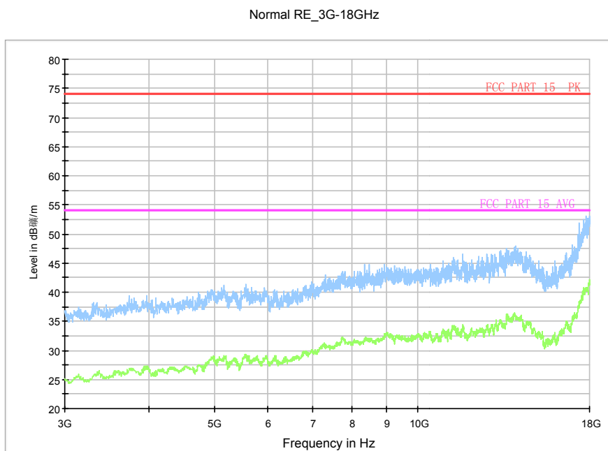
Fig.79. Radiated emission: 8DPSK, Channel 0, 3 GHz - 18 GHz
