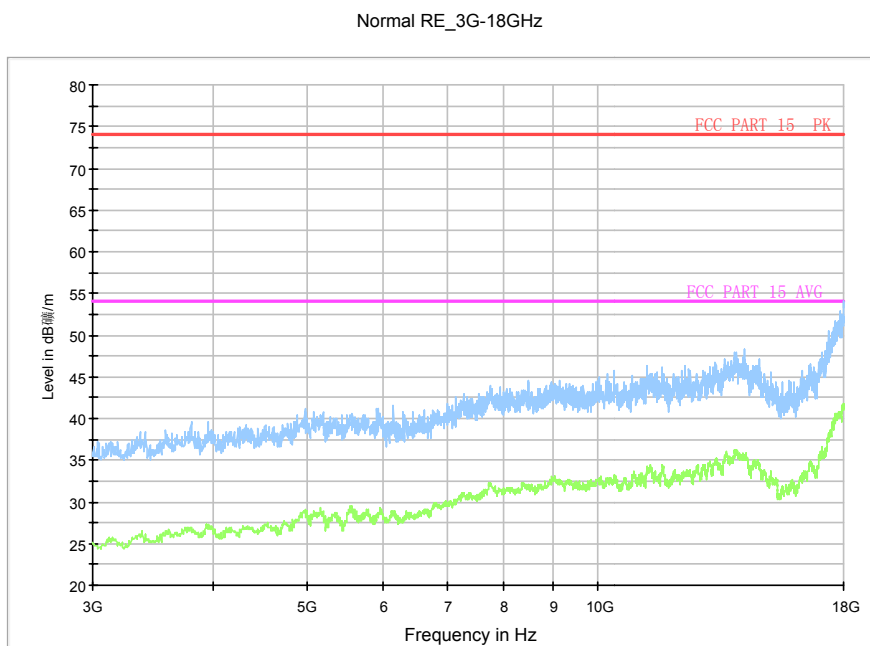
Fig.69. Radiated emission: \pi/4 DQPSK, Channel 0, 3 GHz - 18 GHz
