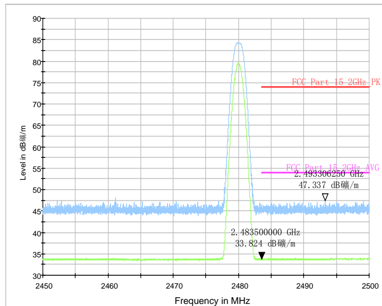
RE-BT-Power_2.45G-2.5GHz
