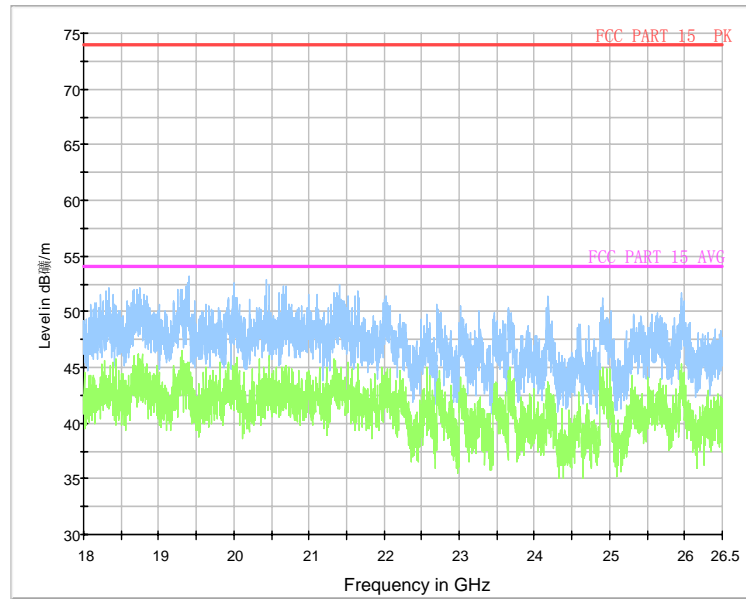
Fig.28. Radiated emission: GFSK, 18 GHz - 26 GHz
