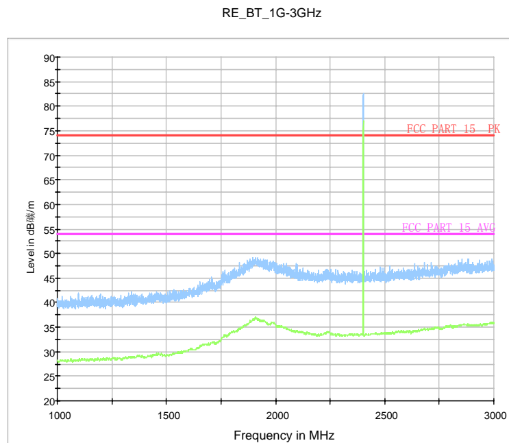
Fig.18. Radiated emission: GFSK, 2402MHz, 1 GHz - 3GHz
