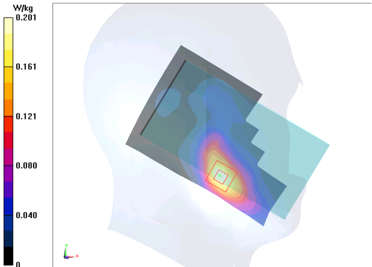
Fig.4 1900 MHz CH810
