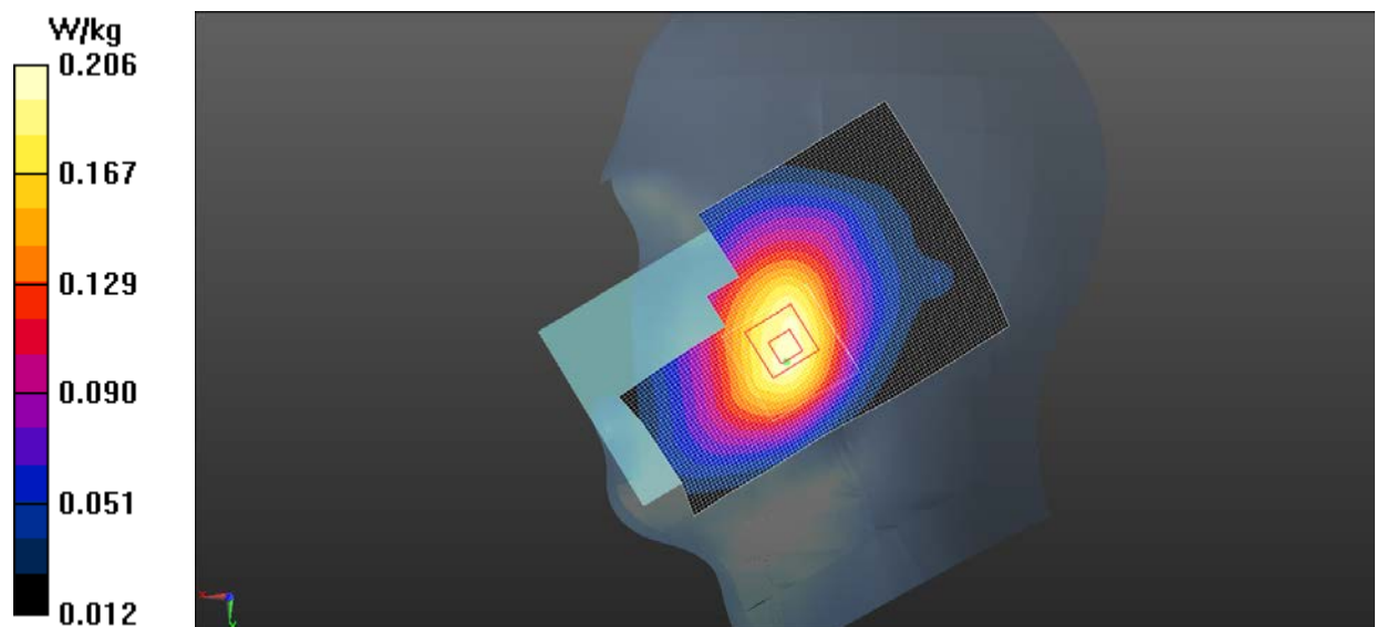
Fig.1 850MHz CH251
