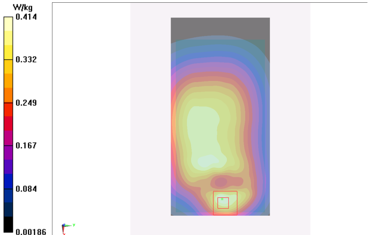
Fig.2 850 MHz CH251
