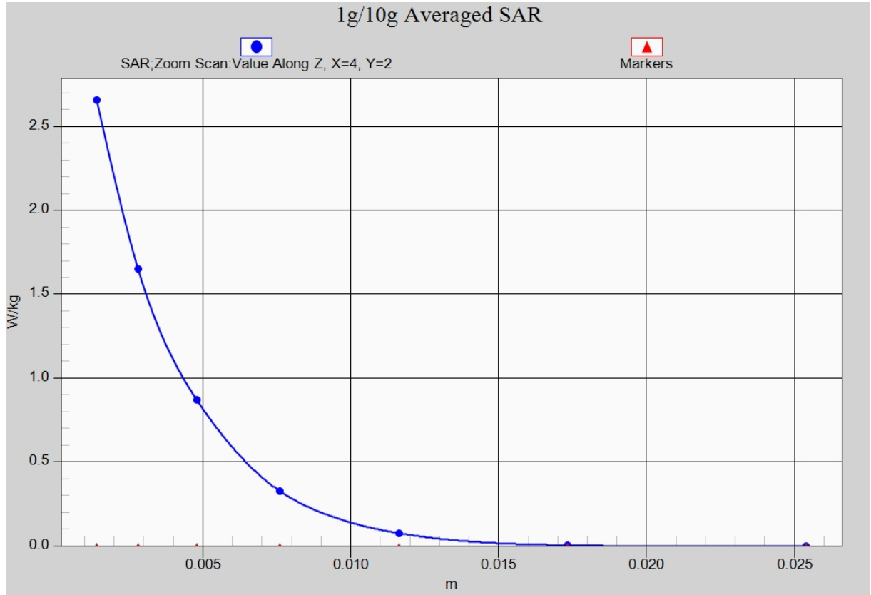
Fig. 17-1 Z-Scan at power reference point (5GHz CH52)
