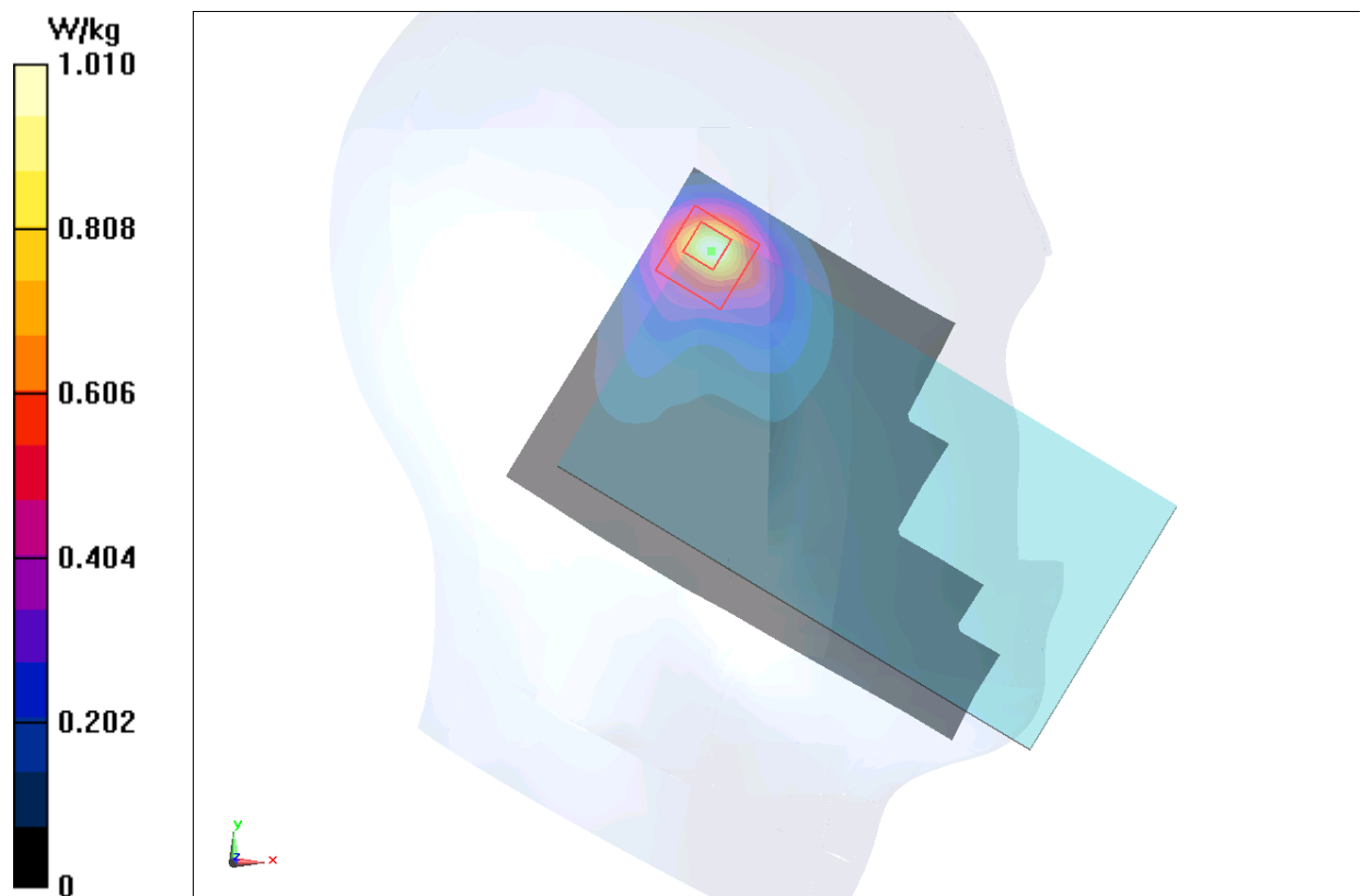
Fig.15 2450 MHz CH1
