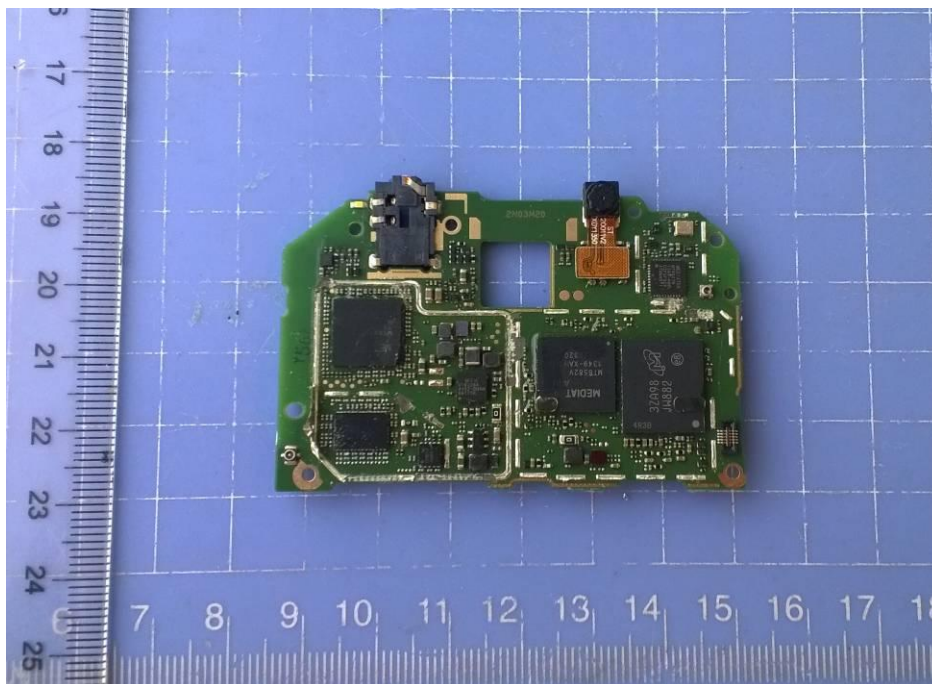
Pic A-8 Mobile phone Disassembly
