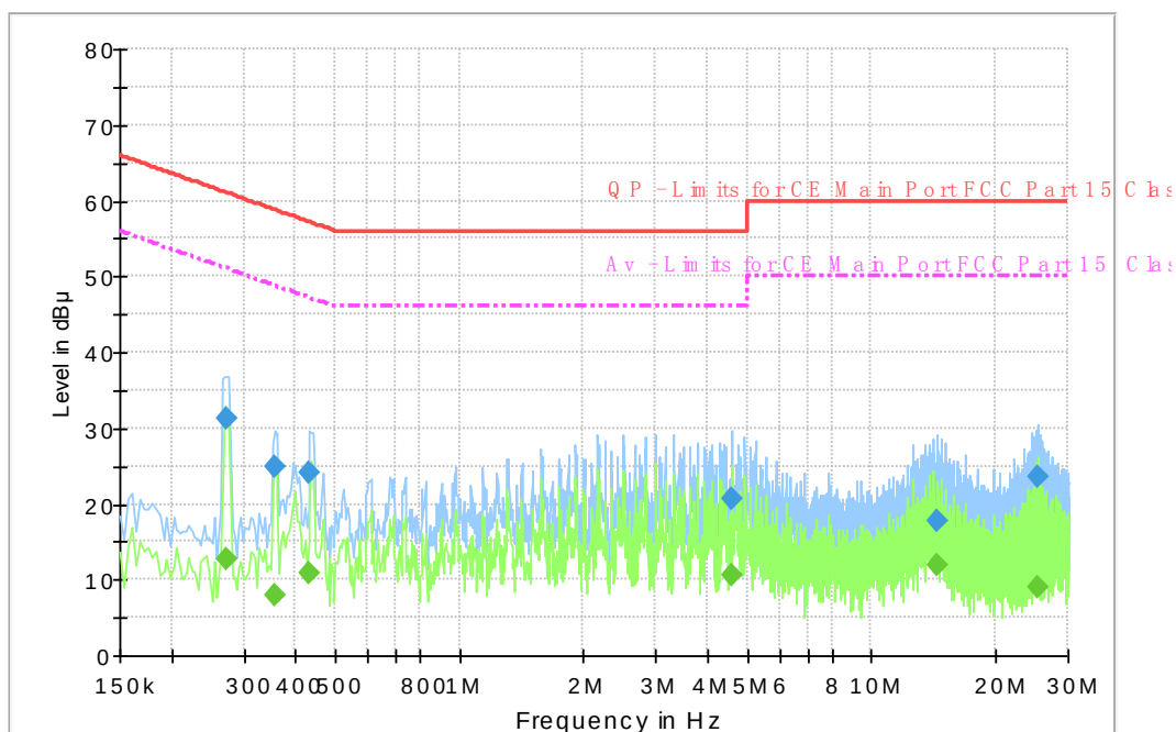
Fig.94 AC powerline Conducted Emission
