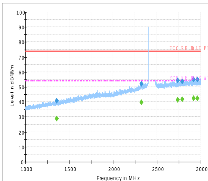
Fig.47 Radiated emission: \pi/4 DQPSK, Ch0, 1GHz~3GHz
