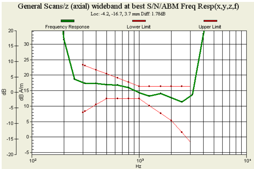
Figure 16 T-Coil GSM 1900 Z Axial
