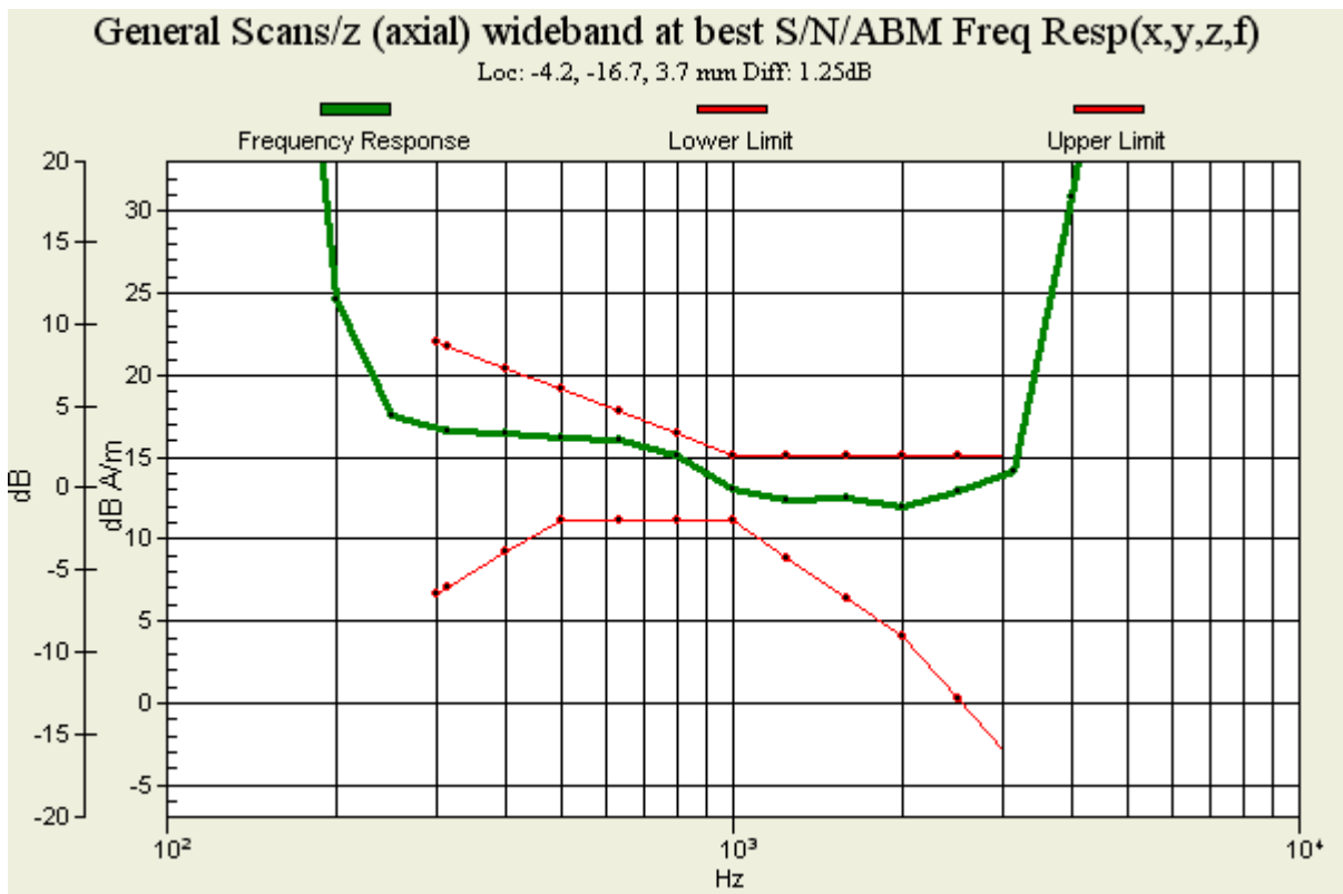
Figure 22 T-Coil WCDMA Band II Z Axial
