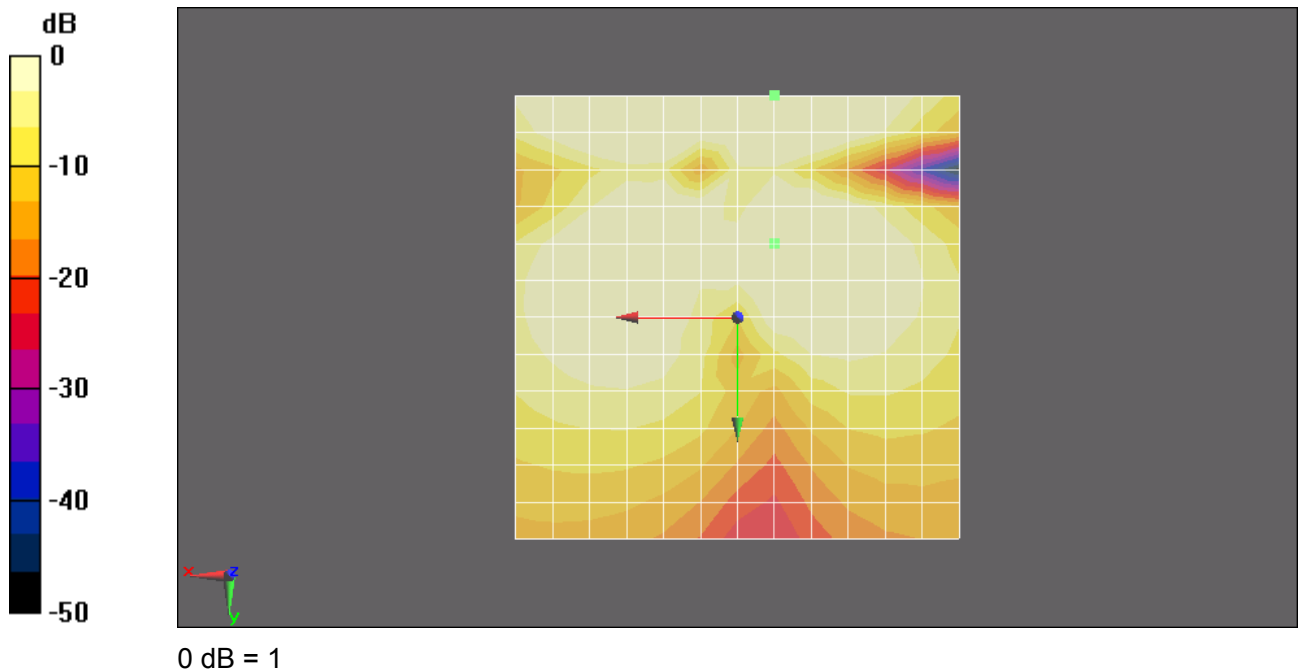
Figure 21 T-Coil WCDMA Band II Y transversal
