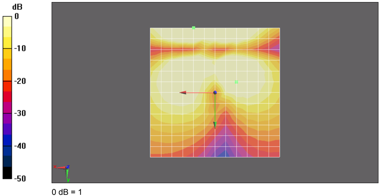
Figure 15 T-Coil GSM 1900 Y transversal
