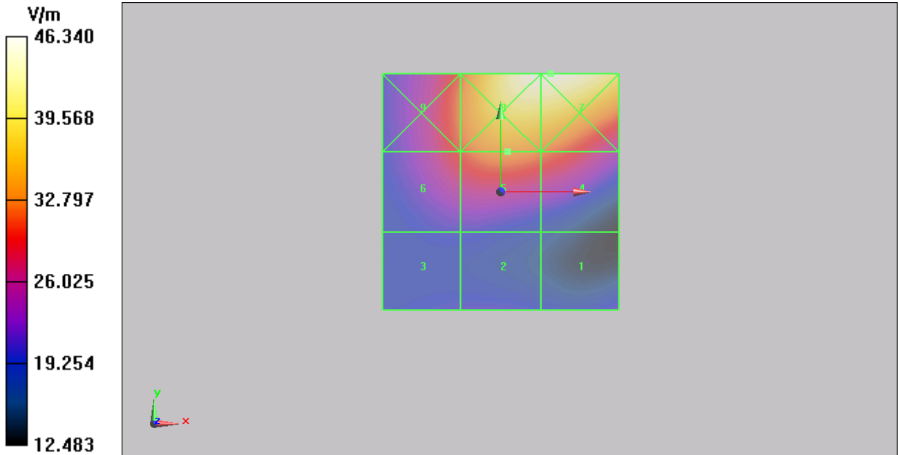
Figure 15 HAC RF E-Field GSM 1900 Channel 661
