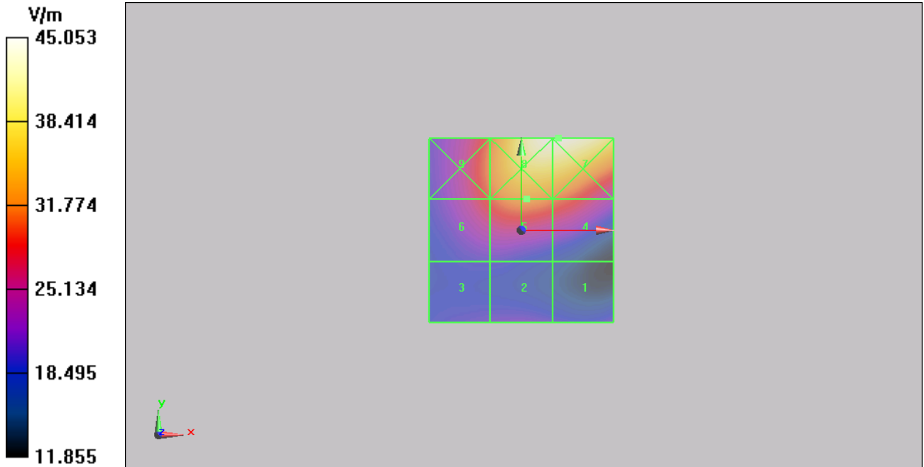
Figure 18 HAC RF E-Field GSM 1900 Channel 661
