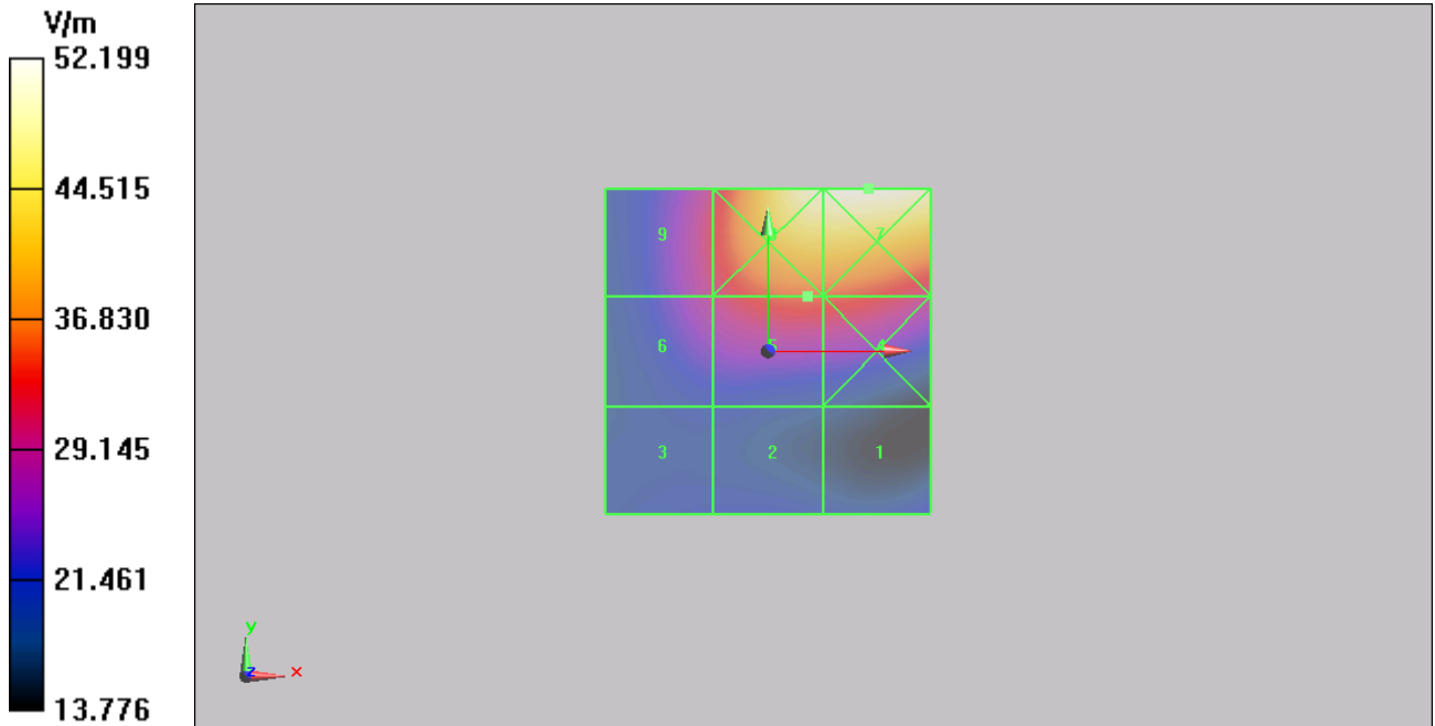
Figure 16 HAC RF E-Field GSM 1900 Channel 512
