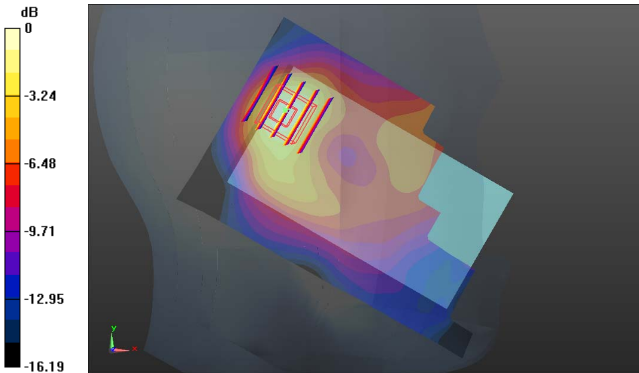
0 dB = 0.110mW/g
