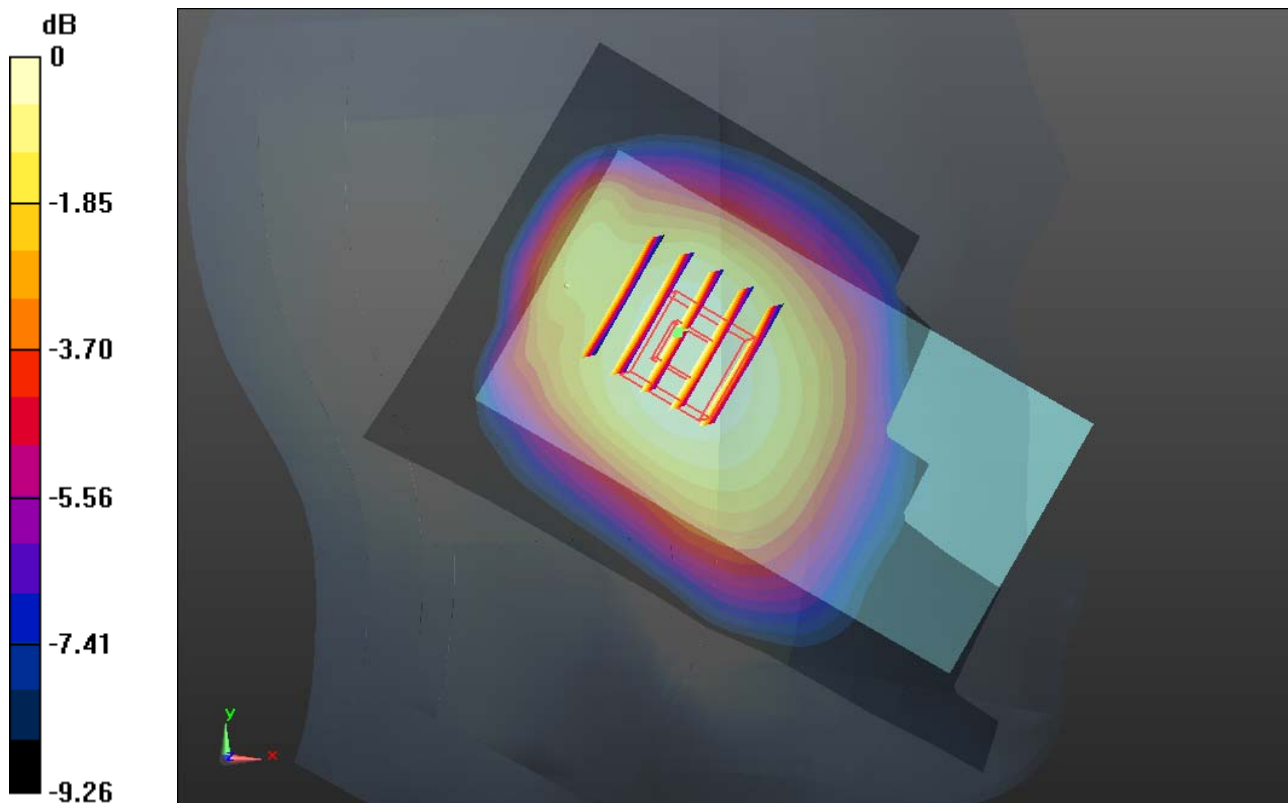
0 dB = 0.140mW/g
