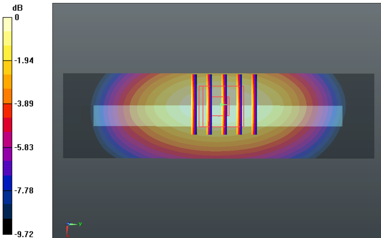
0 dB = 0.230mW/g
