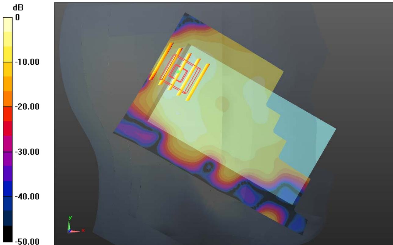
0 dB = 0.090mW/g
