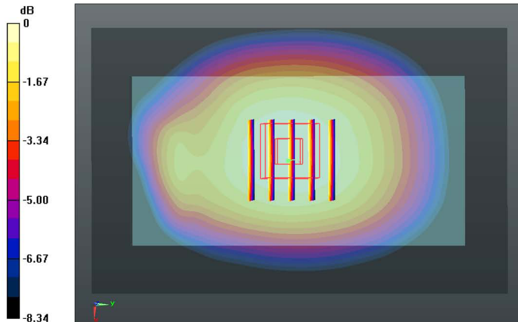
0 dB = 0.310mW/g
