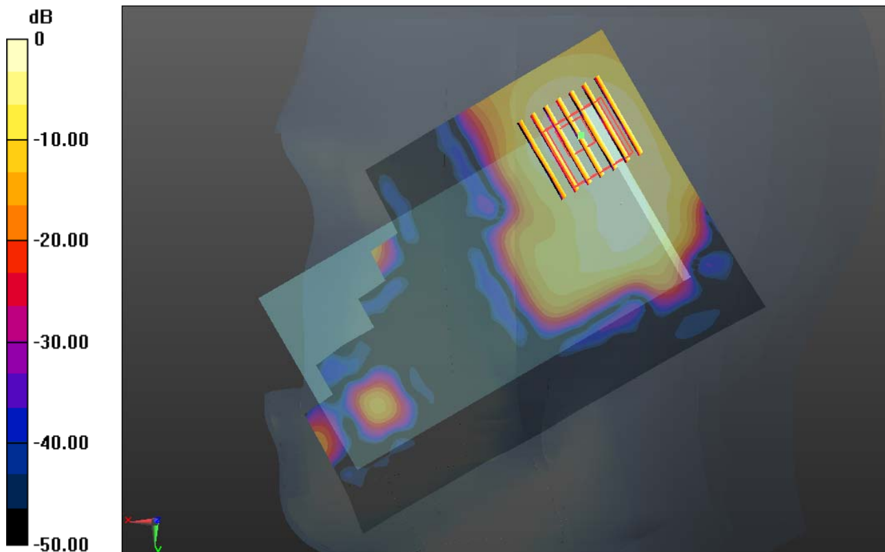
0 dB = 0.210mW/g
