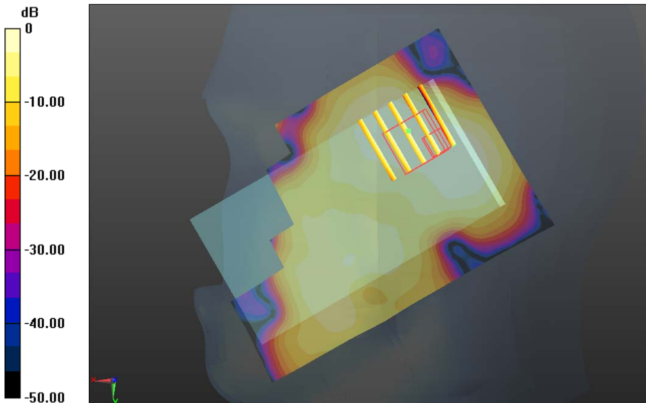
0 dB = 0.070mW/g
