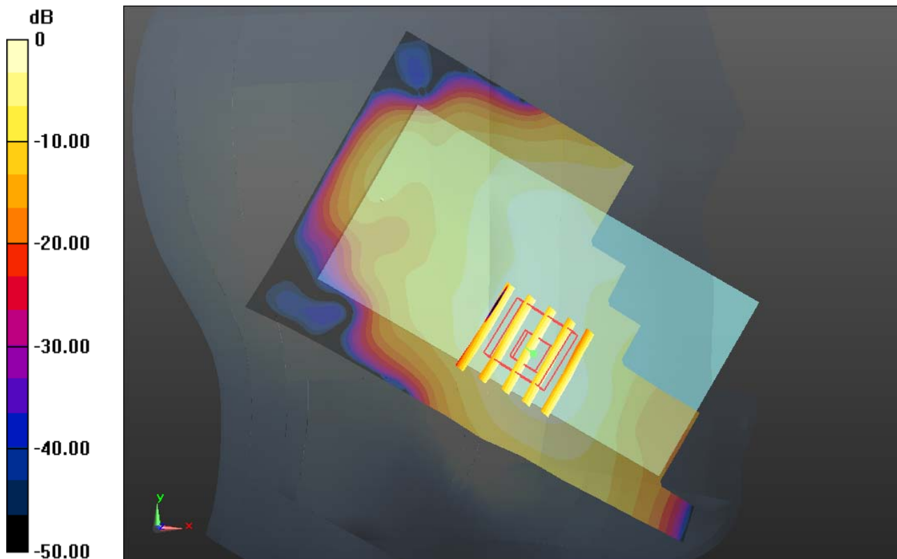
0 dB = 0.130mW/g
