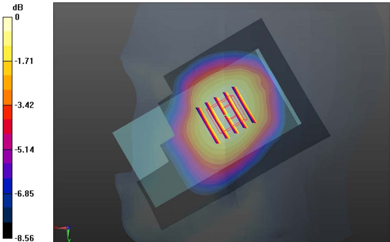
0 dB = 0.120mW/g
