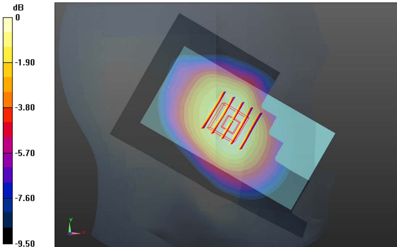
0 dB = 0.180mW/g
