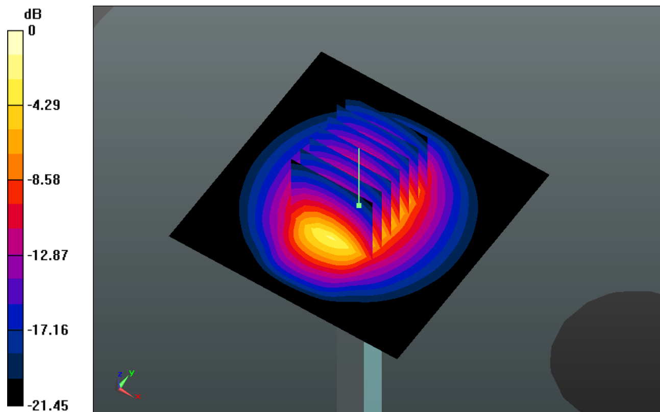
0 dB = 19.160mW/g
