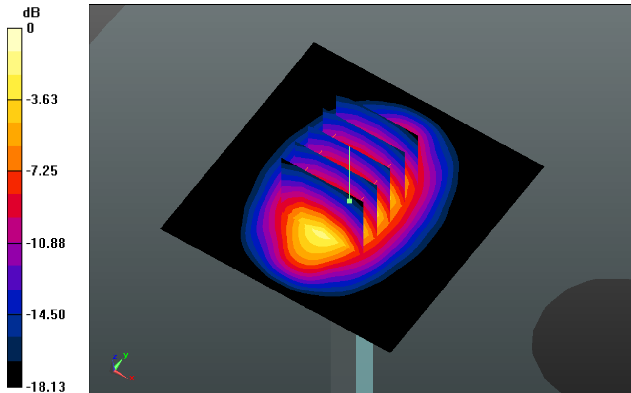
0 dB = 14.480mW/g
