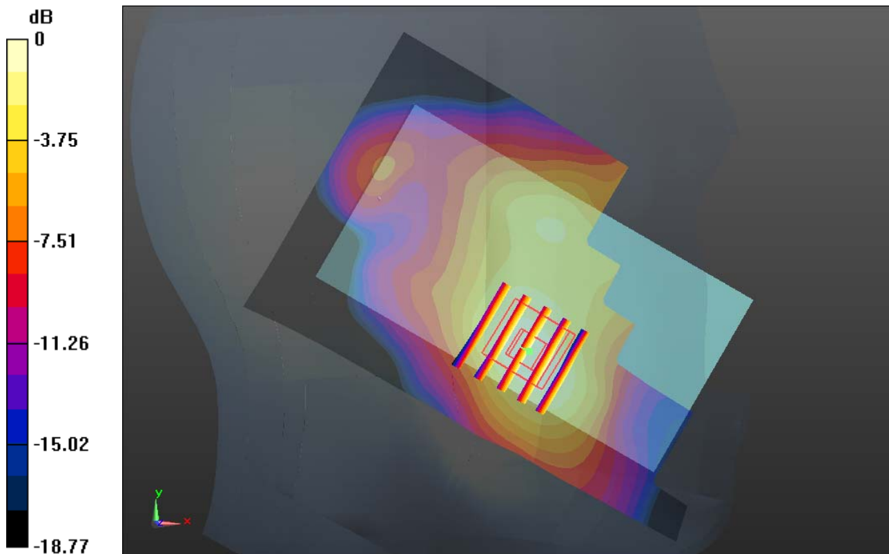
0 dB = 0.310mW/g
