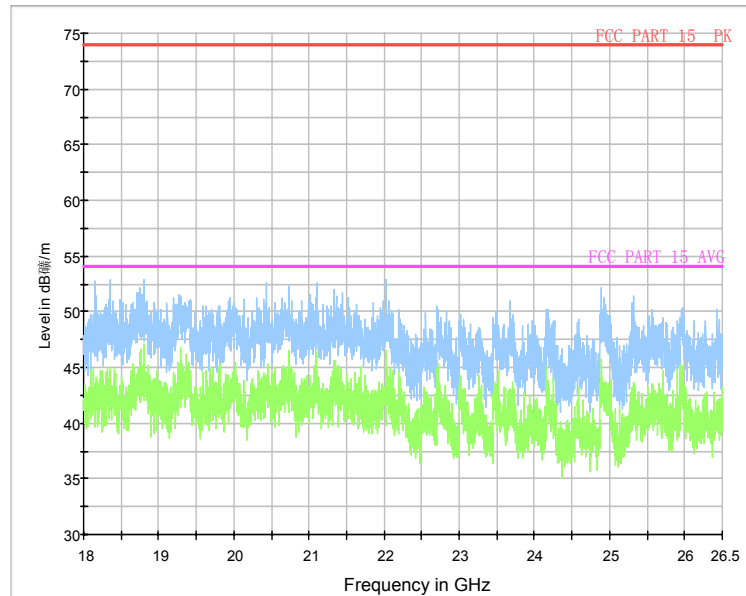
Normal RE_18G-26.5GHz
