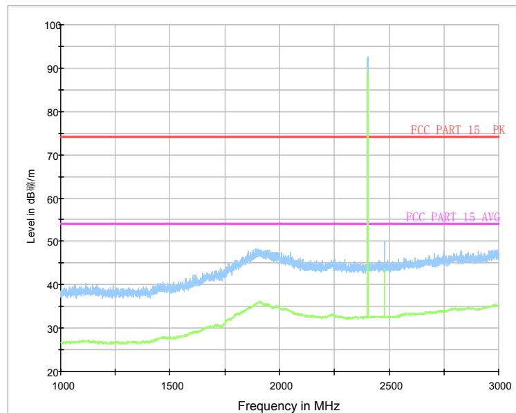
RE_BT_1G-3GHz
