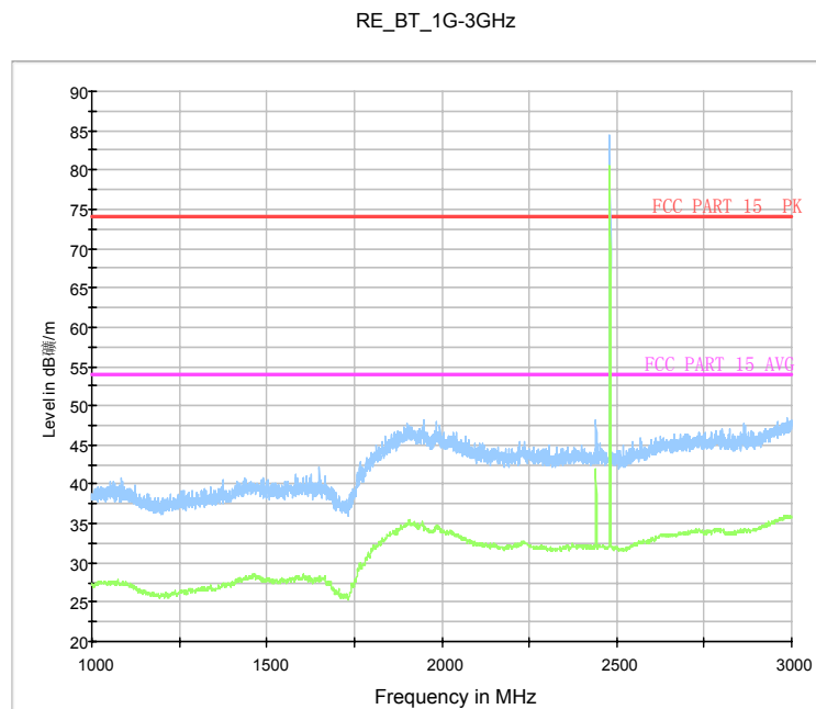
Fig.83. Radiated emission: 8DPSK, Channel 78, 1 GHz - 3 GHz
