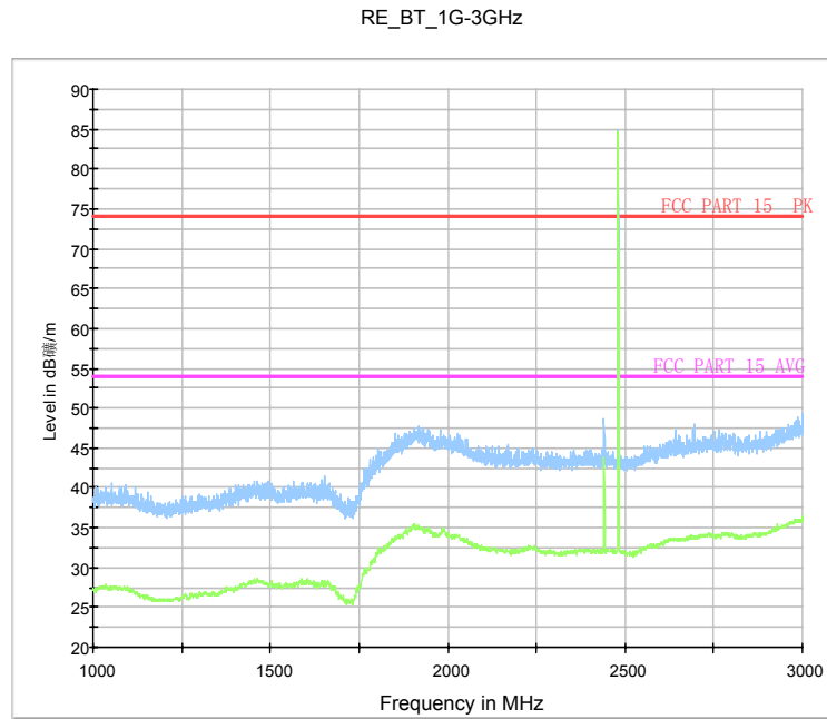
Fig.63. Radiated emission: GFSK, Channel 78, 1 GHz - 3 GHz
