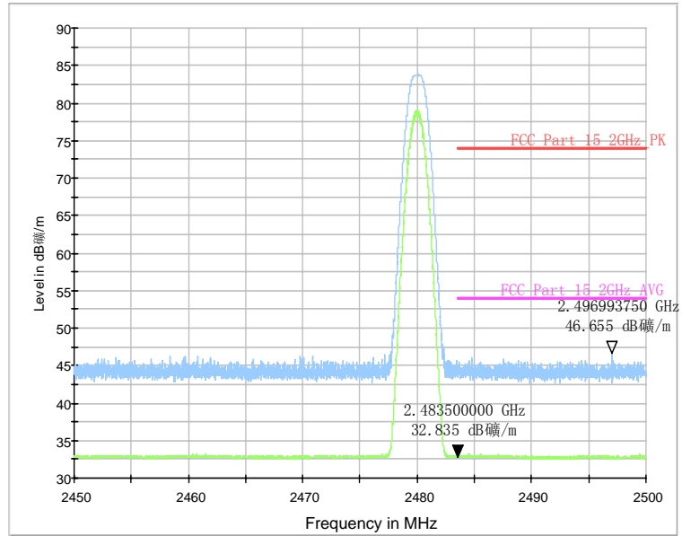
RE-BT-Power_2.45G-2.5GHz
