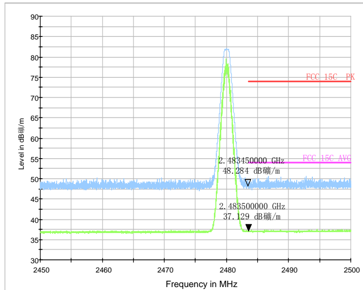
RE-Power_2.45G-2.5GHz
