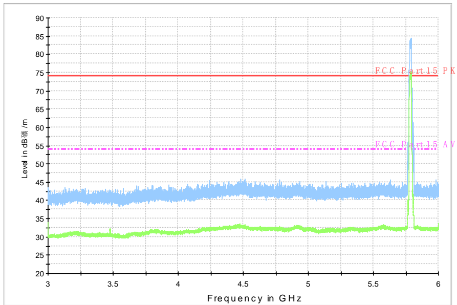
RE - 3GHz-6GHz
