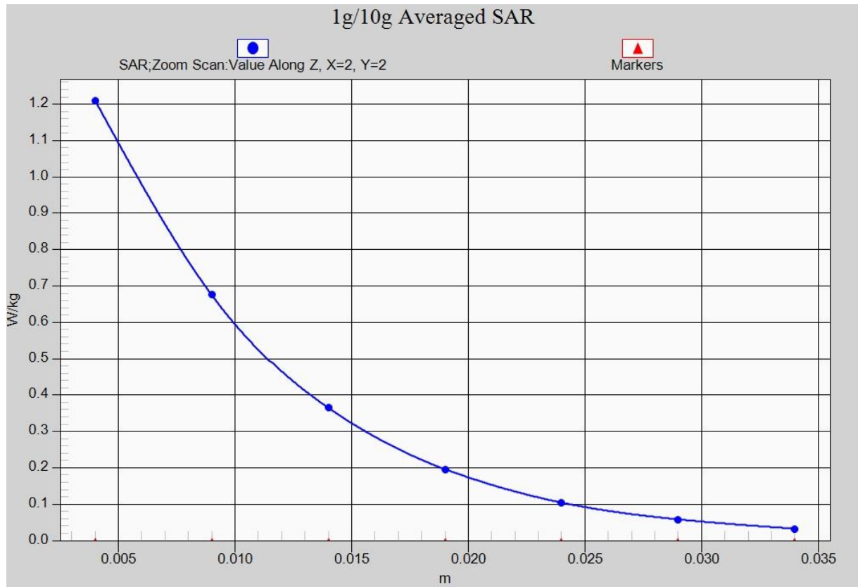
Fig. 8-1 Z-Scan at power reference point (LTE Band7 CH20850)
