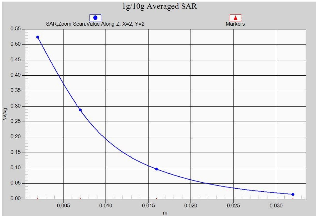
Fig. 7-1 Z-Scan at power reference point (LTE Band7 CH20850)
