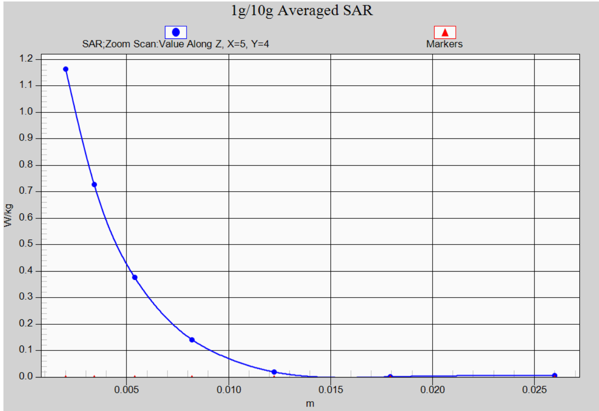
Fig. 11-1 Z-Scan at power reference point (5GHz CH36)
