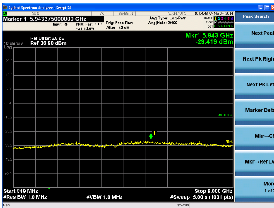
Channel 189, 849MHz~9GHz
