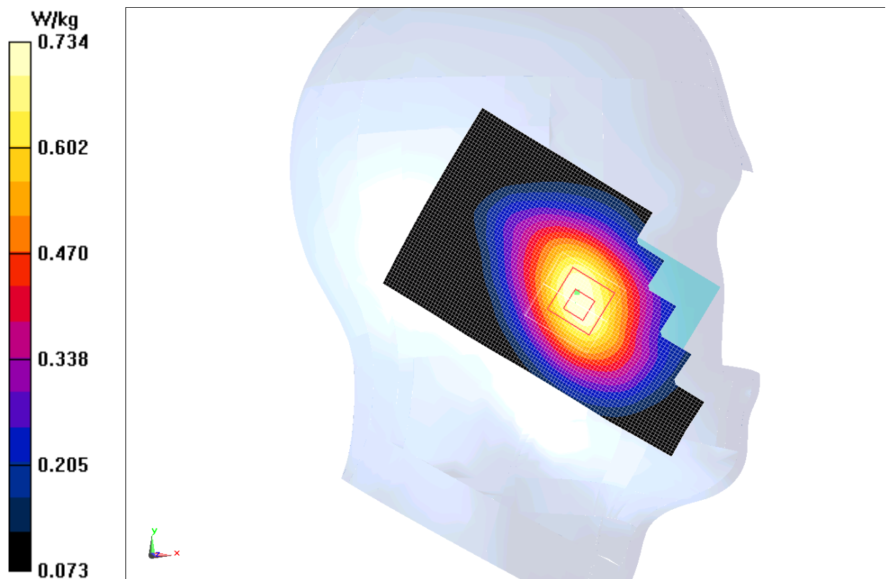
Fig.I.5 WCDMA 850 CH4233
