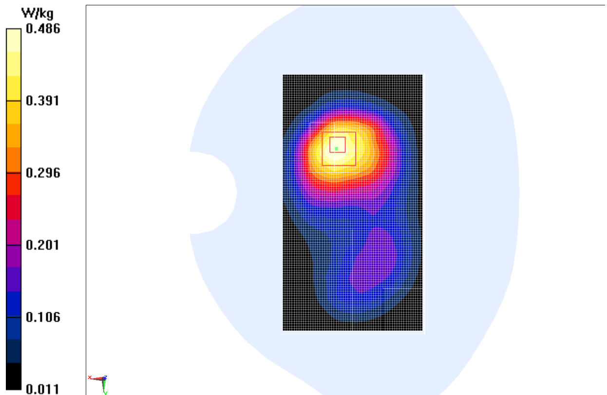
Fig.I.4 1900 MHz CH512
