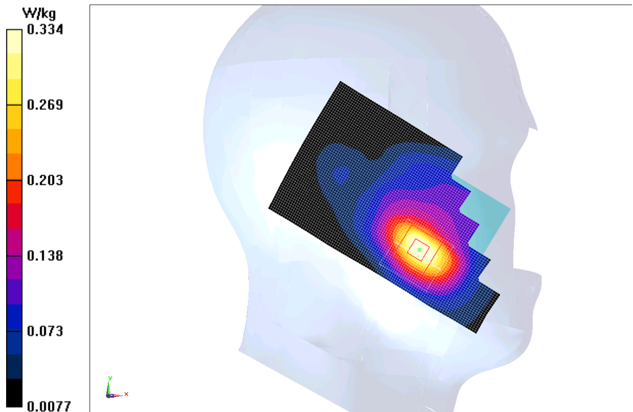
Fig.I.3 1900 MHz CH810
