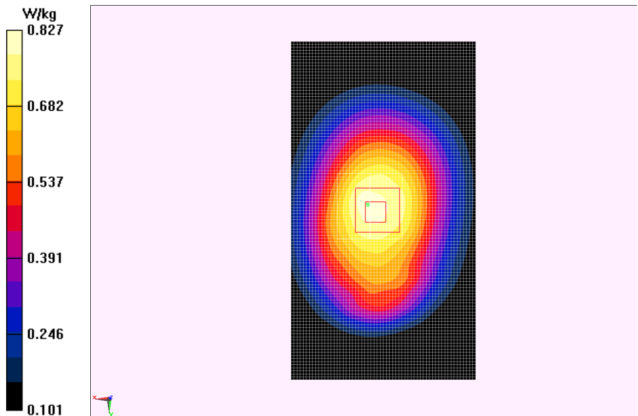
Fig.I.6 WCDMA 850 CH4233
