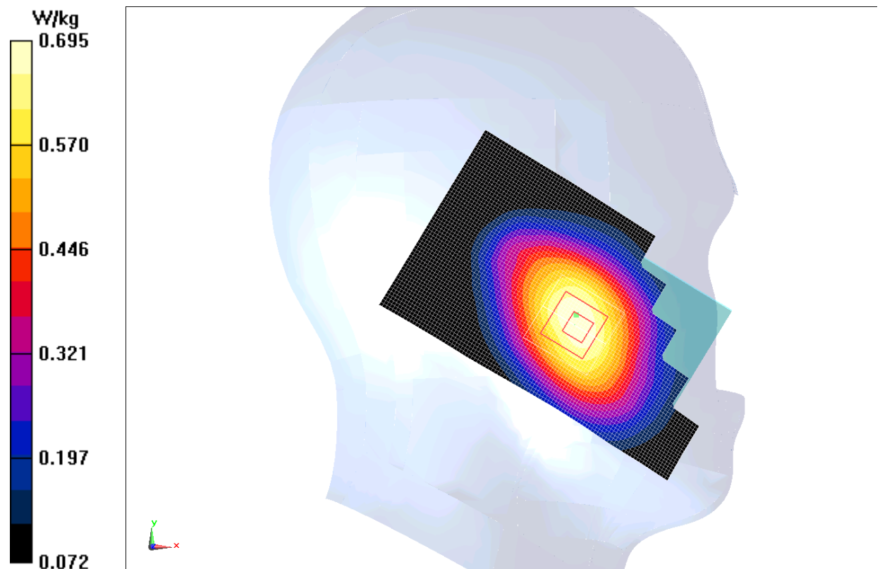
Fig.I.1 850MHz CH251
