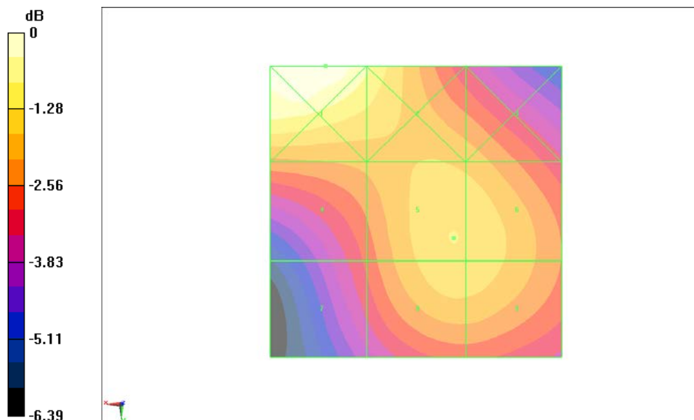
Fig B.23 HAC RF H-Field WCDMA 1900 Middle
