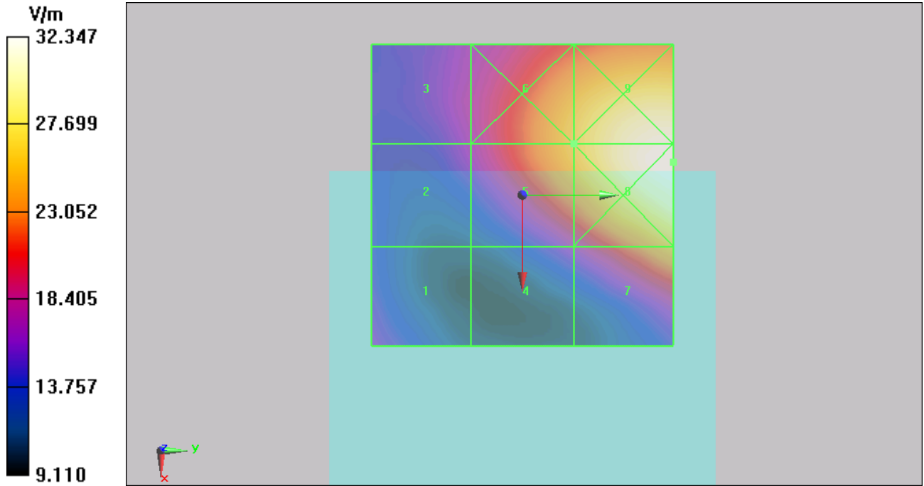
Figure 19 HAC RF E-Field GSM 1900 Channel 512
