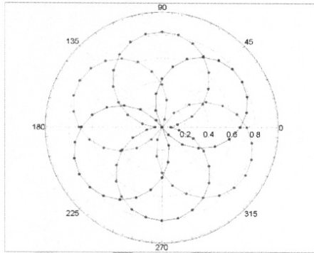
f=600 MHz,TEM
