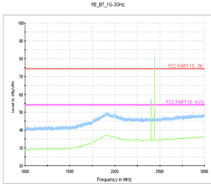
Fig.81. Radiated emission: 8DPSK, Channel 39, 1 GHz - 3 GHz
