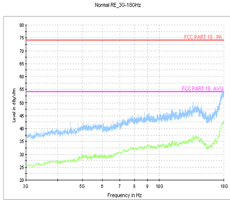
Fig.59. Radiated emission: GFSK, Channel 0, 3 GHz - 18 GHz
