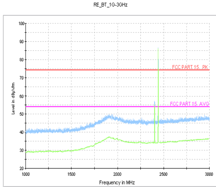
Fig.61. Radiated emission: GFSK, Channel 39, 1 GHz - 3 GHz
