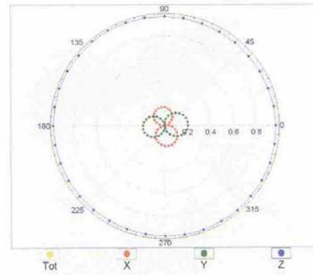
f=2500 MHz,R22,90°
