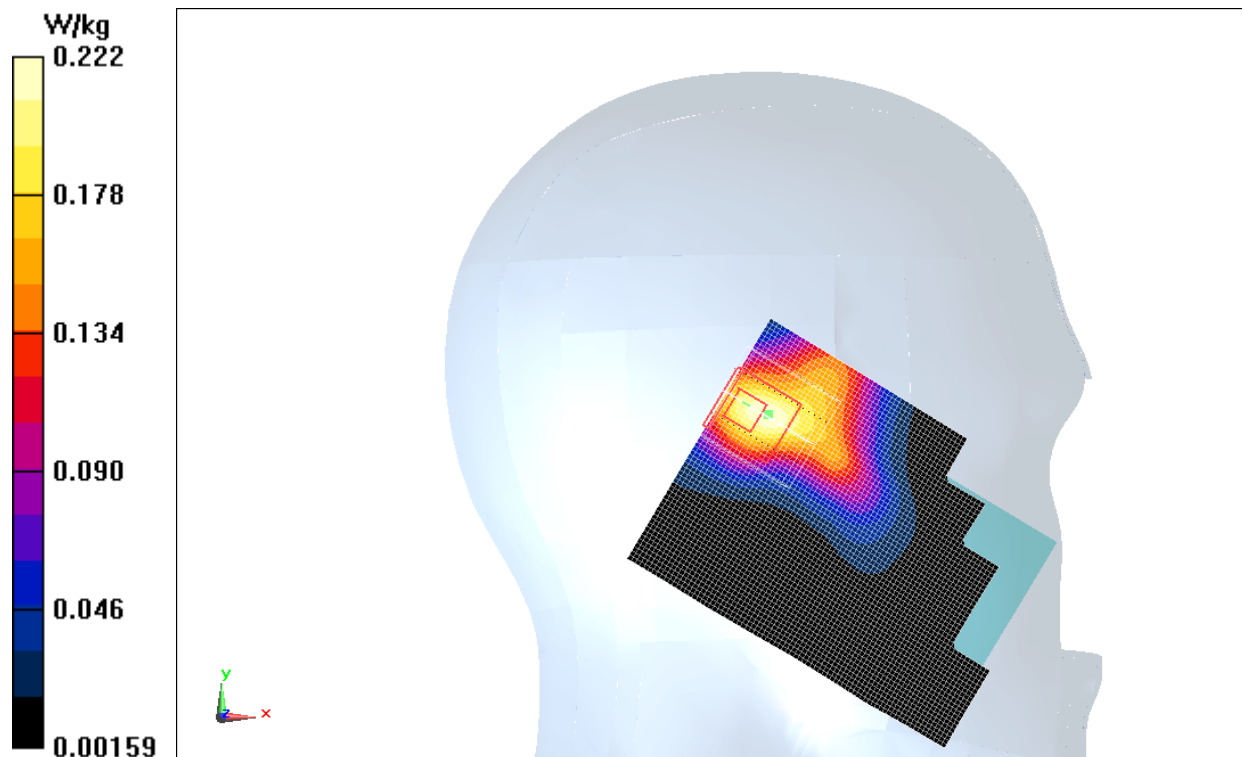
Fig.9 2450 MHz CH11
