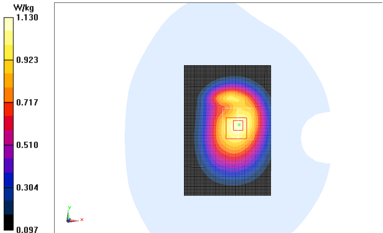
Fig.6 WCDMA 850 CH4132
