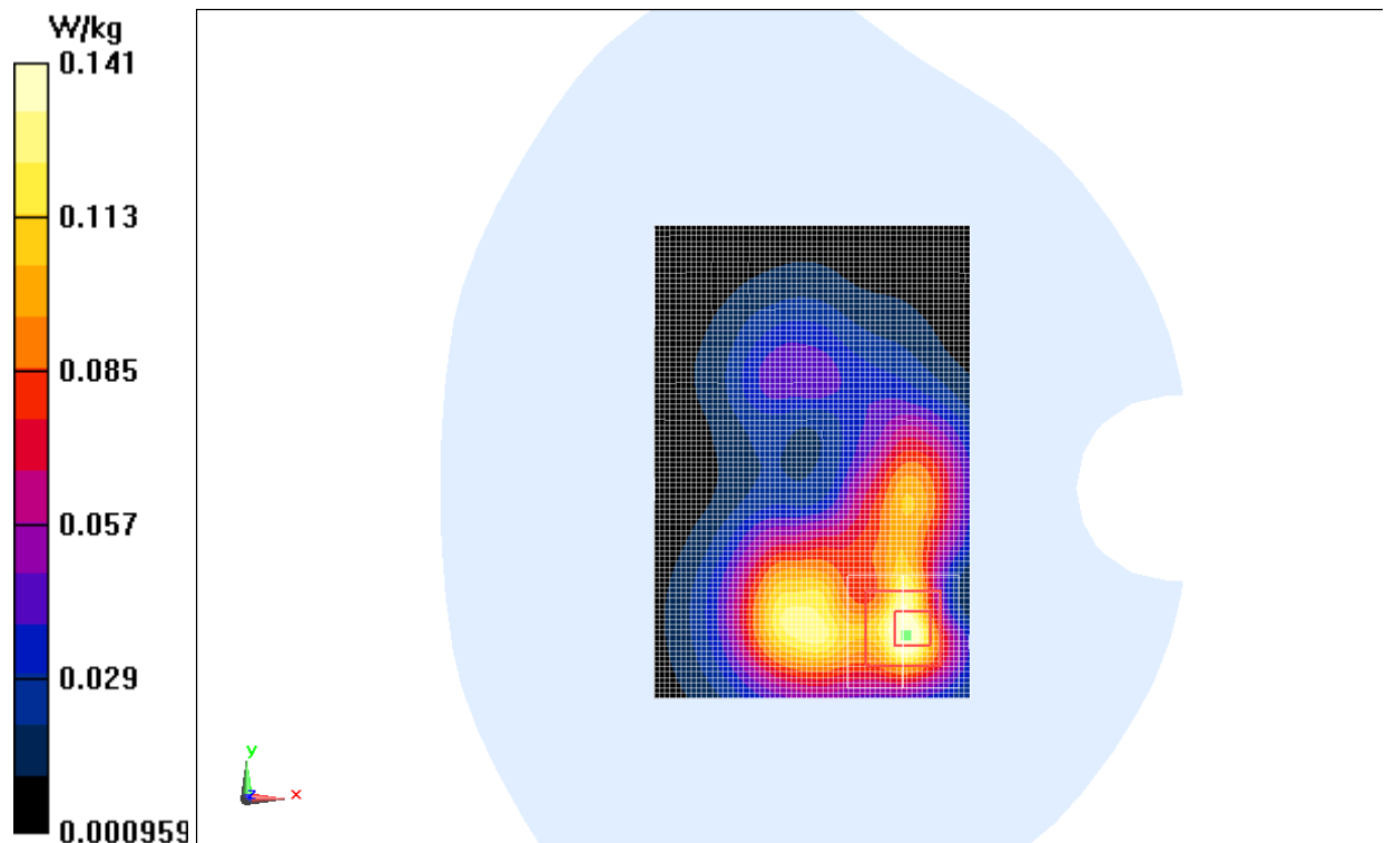
Fig.10 2450 MHz CH11
