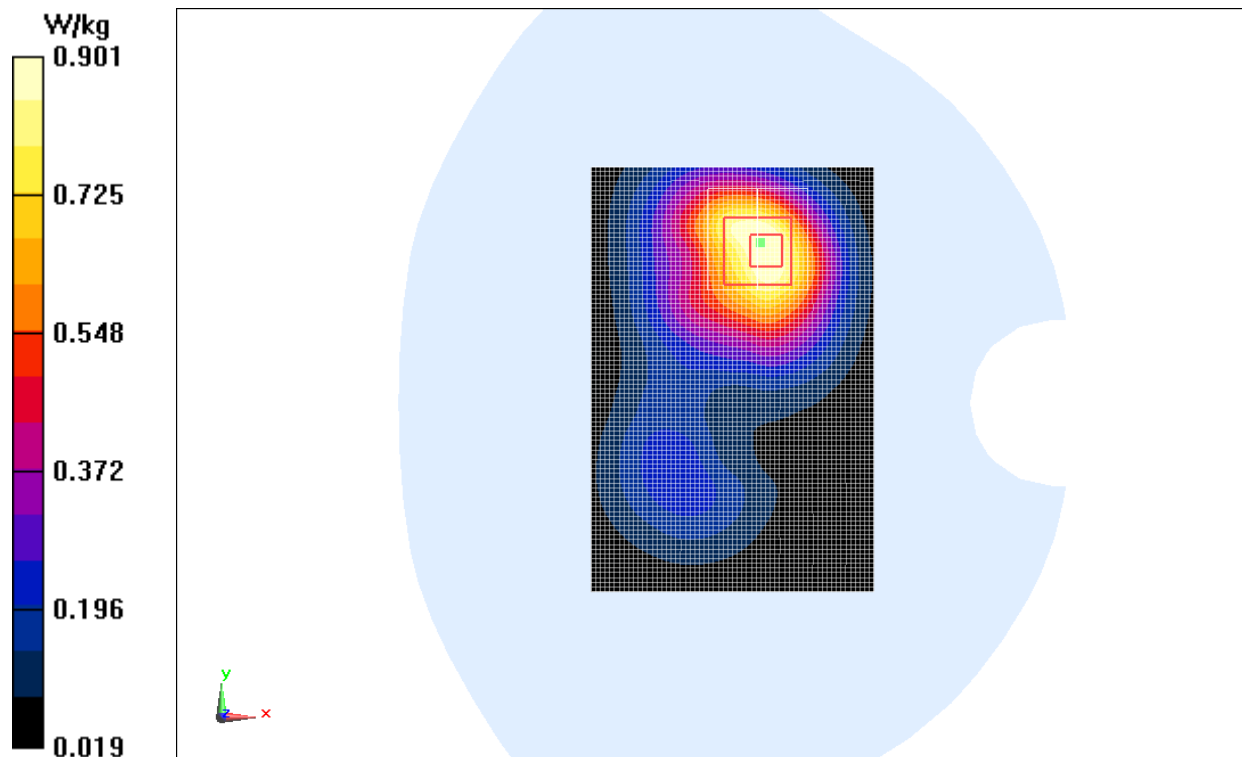
Fig.4 1900 MHz CH810
