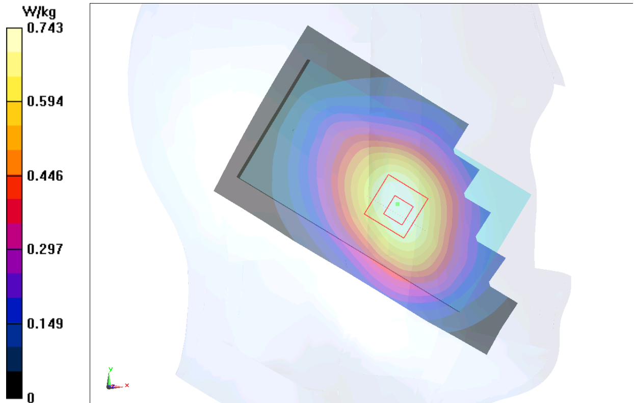
Fig.5 WCDMA 850 CH4132
