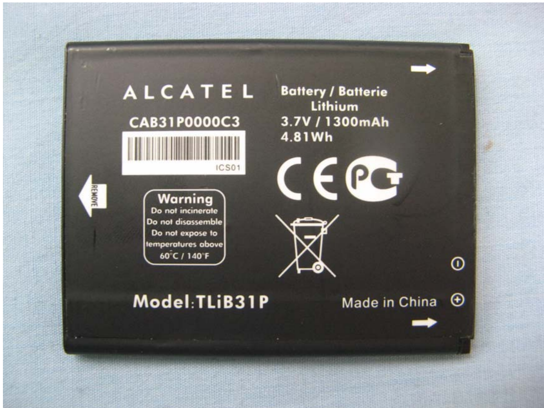
Battery AE2
