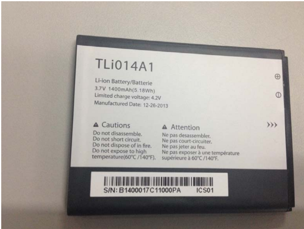
Battery AE2
