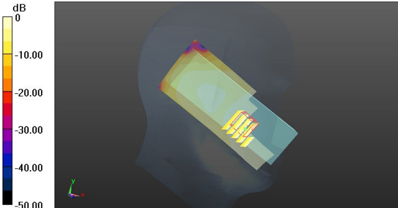
0 dB = 0.0562 \text{ W/kg}
