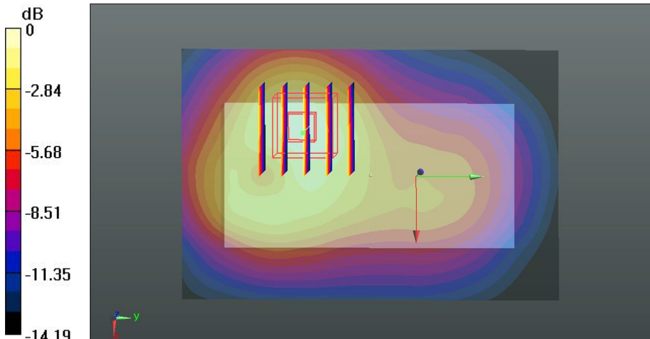
0 dB = 0.401 \text{ W/kg}
