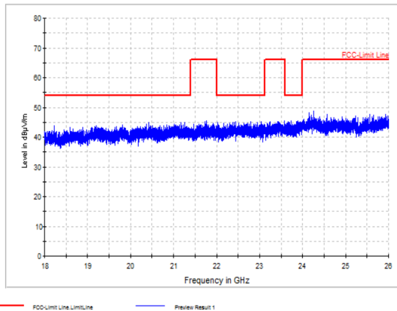
Fig.69. Radiated emission: GFSK, 18 GHz - 26 GHz
