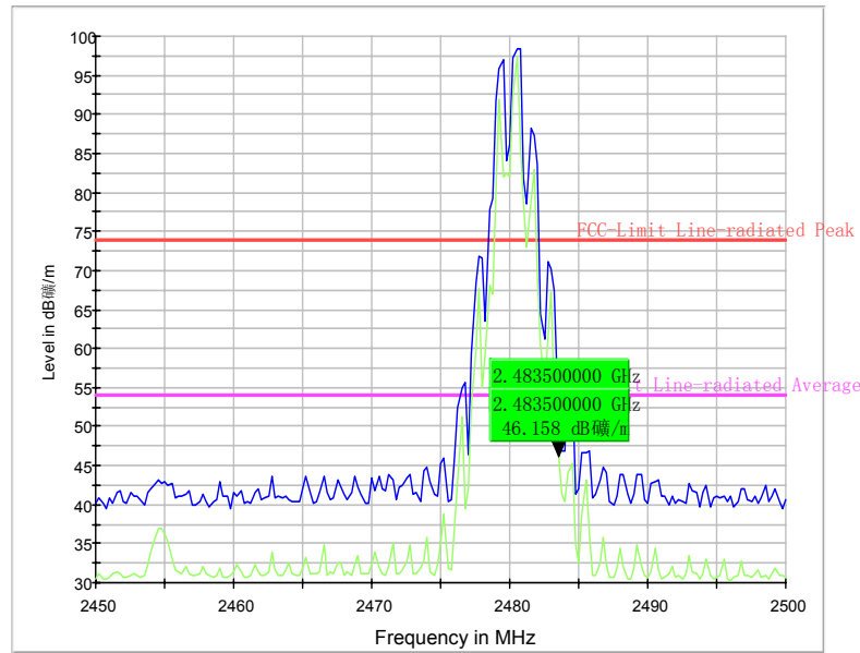
FCC-RE2-1-18G-PEAK+AV
