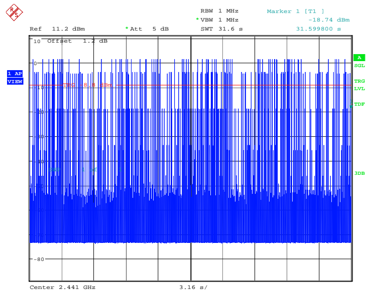
Fig.104. Time of occupancy (Dwell Time): Channel 39, Packet 2-DH5
