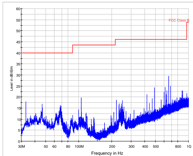
FCC Part15 30MHz-1GHz
