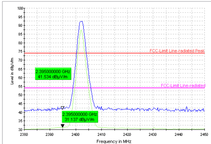
FCC-RE2-1-18G-PEAK+AV
